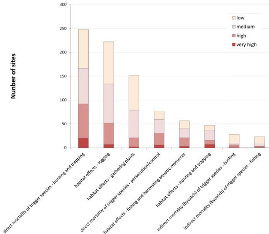
Figures 9c. Level 2 threats associated with over-exploitation, persecution and the control of species.
