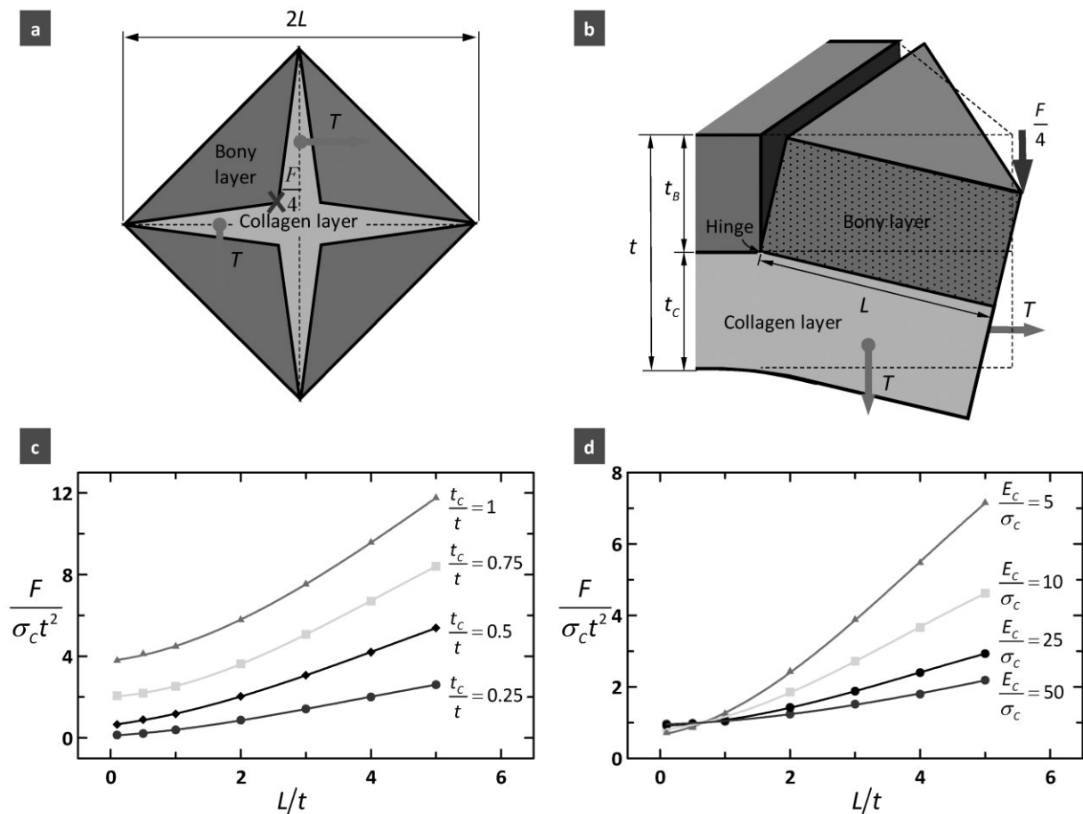
Fig. 6. (a) Top view of the idealized puncture configuration; (b) three-dimensional view of single bony flaps. The force applied by the needle ( F/4 ) and the forces generated by the tension in the collagen layer are shown. (c) Effect of collagen layer thickness and (d) collagen resilience on the normalized penetration force.
