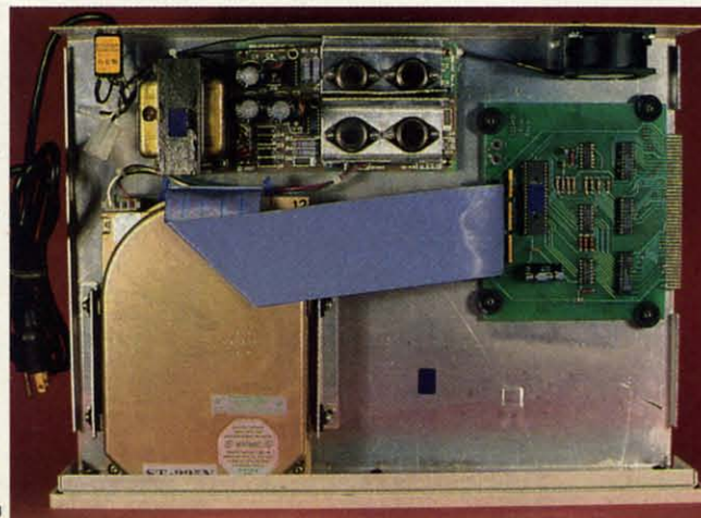
The A20 is built around a Seagate ST225N SCSI hard drive module (bottom) with its own power supply (top) and Amiga to SCSI interface (right).
