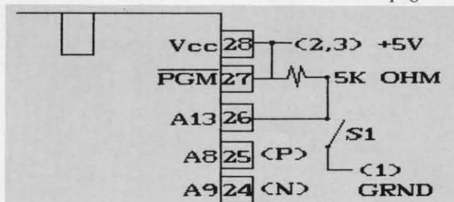
Figure 4: Modification for Bank Switching a 27128 EPROM S1 Closed = Bottom 8K S1 Open = Top 8K
