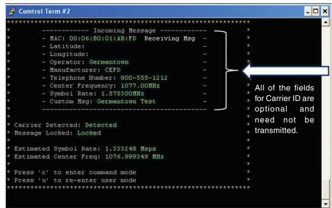
Figure 2, Decoded Carrier ID Format.
