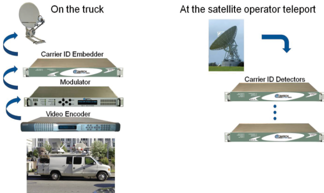
Figure 4, Carrier ID Implementation Topology – SNG Video.
