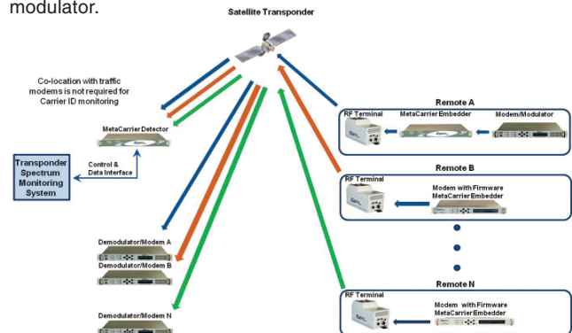
Figure 3, Carrier ID Implementation Topology – SCPC Network.
