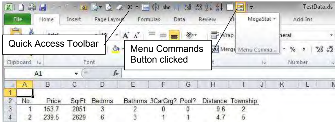
Figure 13 Accessing MegaStat from the Quick Access Toolbar.
