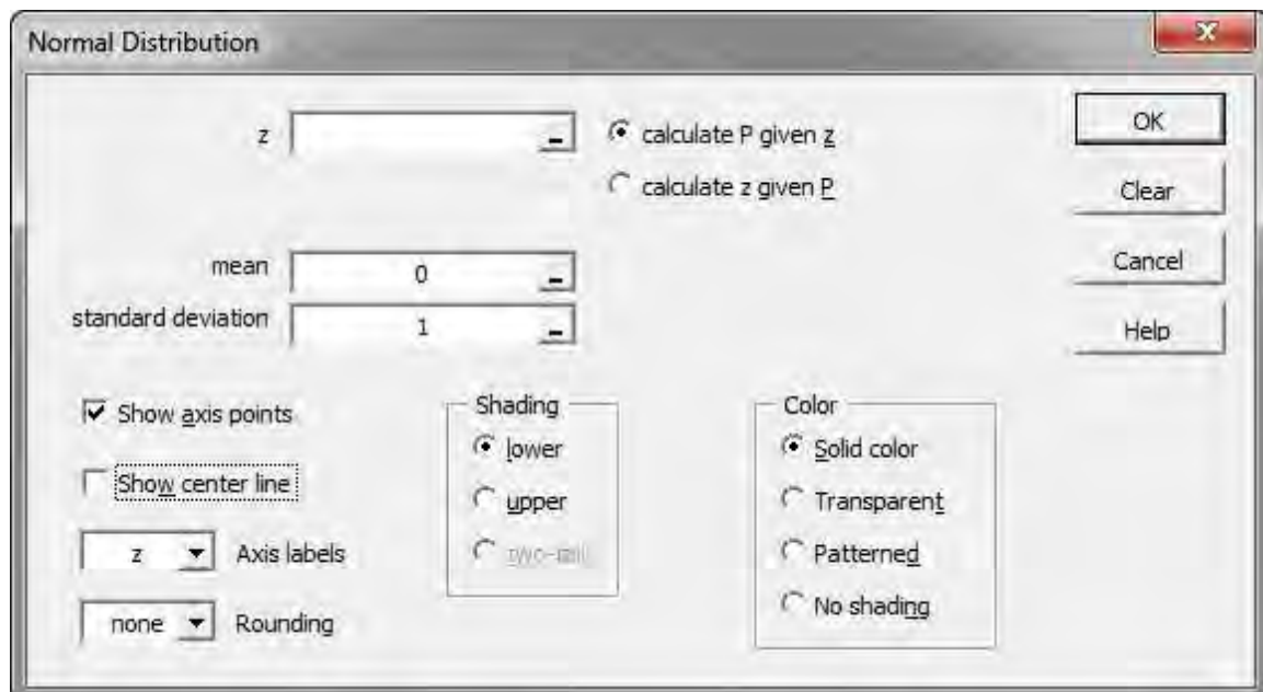
Figure 10a. Normal distribution dialog box.
