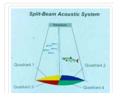
Split beam transducer receives echoes with four different
