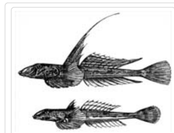
Callionymus
