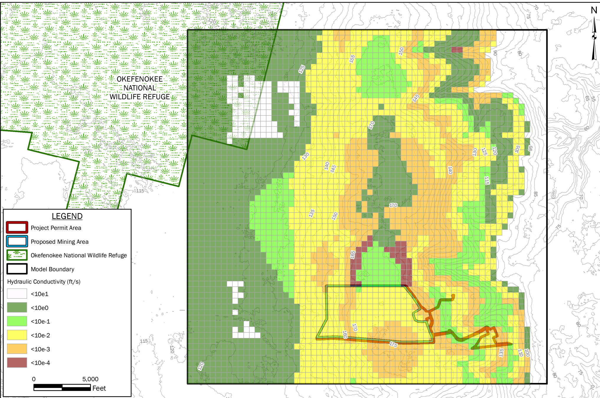
FIGURE 50: CALIBRATED MODEL HORIZONTAL HYDRAULIC CONDUCTIVITY LAYER 8 TWIN PINES MINERALS ST. GEORGE, CHARLTON COUNTY, GEORGIA
