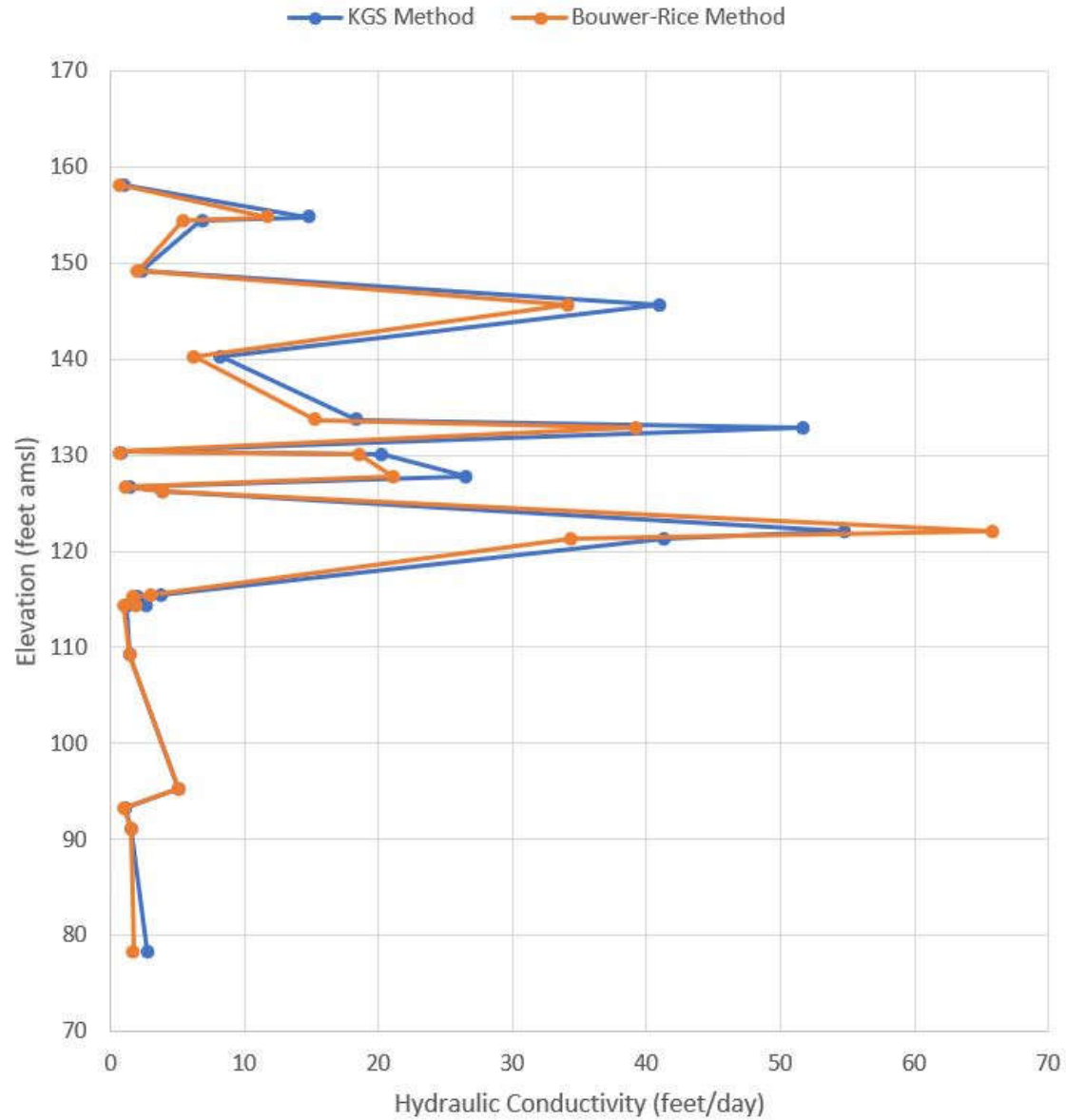
FIGURE 19: SLUG TEST HYDRAULIC CONDUCTIVITY V. ELEVATION
