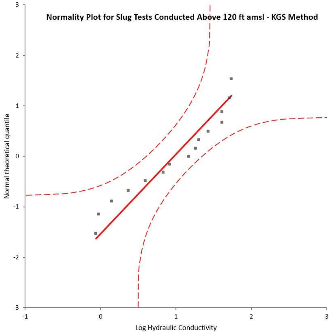
FIGURE 20: SLUG TEST NORMALITY PLOT (ABOVE 120 FT AMSL)
