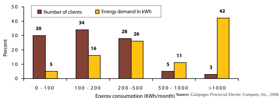
Figure 5. Distribution of clients and total energy demand in kWh by range of consumption in Santa Cruz
