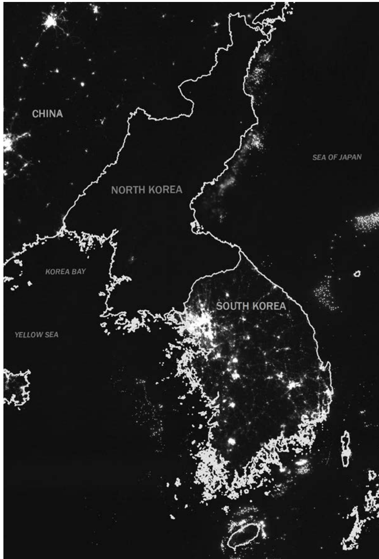
Satellite view of the Korean Peninsula at night, 2020. Visible light emissions from North Korea continue to be extremely sparse, reflecting limited availability of electricity to most of the country outside the capital, Pyongyang, and the leadership's fundamental decision to invest a large portion of North Korea's resources into building military power.
