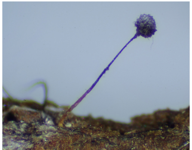
This tiny 1.1 mm high Macbrideola sp. was found on the same substrate as Calomyxa metallica .
