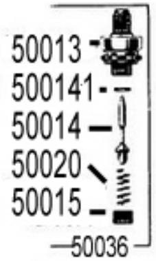
Air Valve Assembly, All
