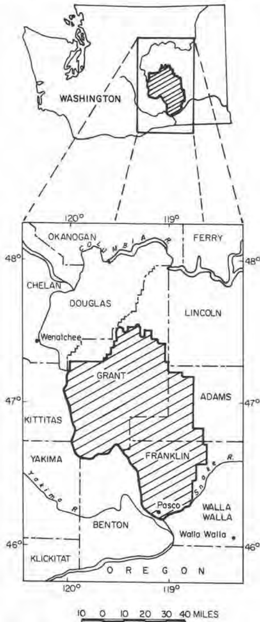
FIGURE 1.—Location of the project area.
