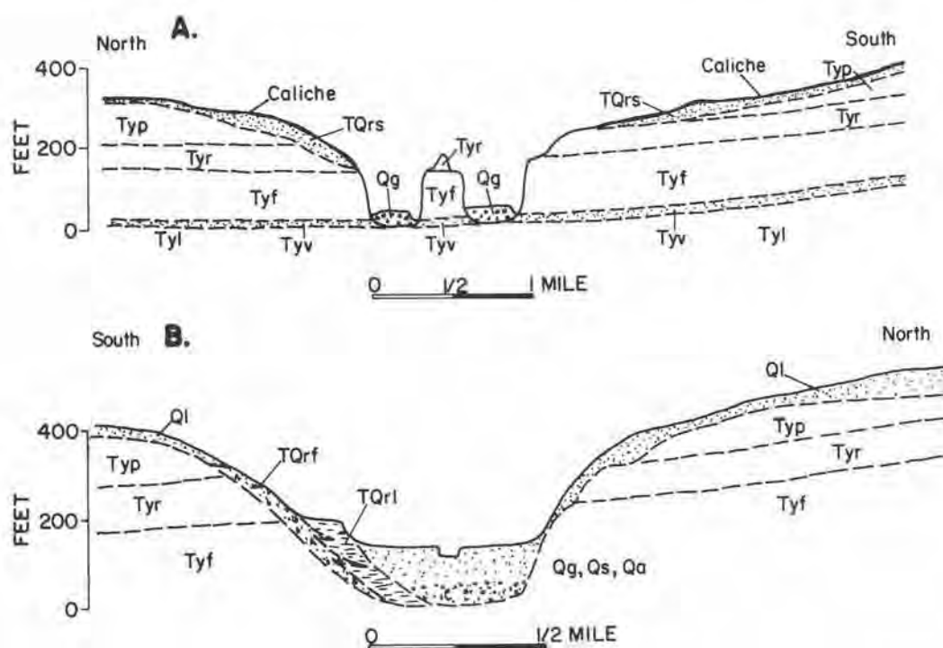
FIGURE 22.—Diagrammatic sections across (A) Potholes Coulee and (B) Lind Coulee near Providence, showing unconformable relationships. Tyl, lower Yakima Basalt (flows below the Vantage Sandstone Member); Tyv, Vantage Sandstone Member; Tyf, Frenchman Springs Member; Tyr, Roza Member; Typ, Priest Rapids Member; TQrf, Ringold fan conglomerate; TQrl, Ringold lacustrine clay and silt; TQrs, Ringold tuffaceous sand; Ql, loess; Qg, Qs, Qa, fluvial gravel and sand (flood deposits) and alluvium.
