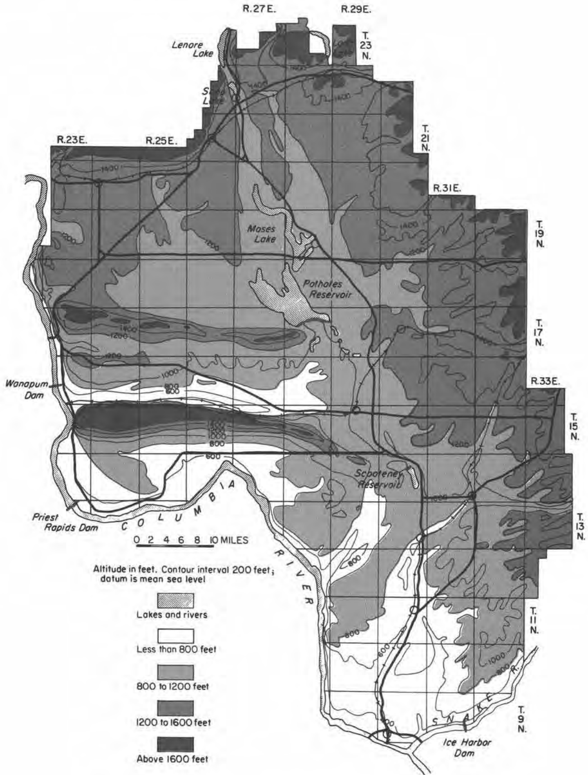
FIGURE 3.— Generalized land-surface altitudes within the project area.
