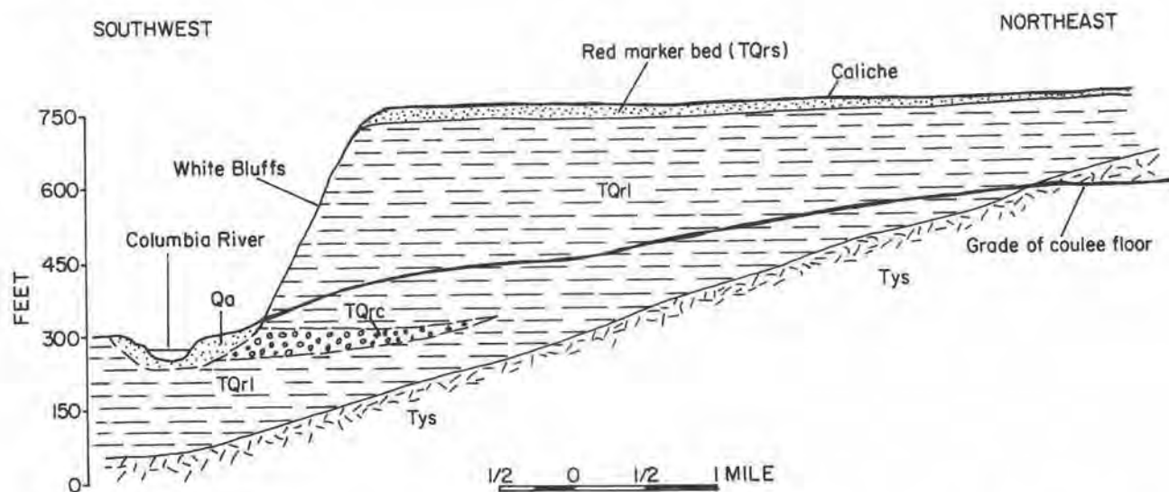
FIGURE 20.—Diagrammatic section showing unconformable relationships along Ringold Coulee. Tys, Saddle Mountains Member; TQrl, Ringold lacustrine clay and silt; TQrc, Ringold conglomerate; TQrs, Ringold tuffaceous sand; Qa, alluvium.
