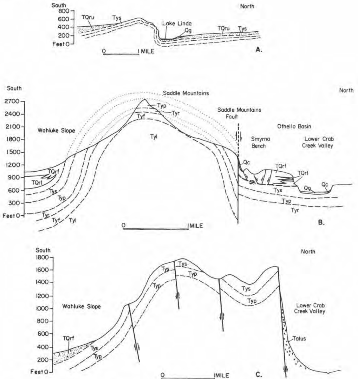
FIGURE 31.—Diagrammatic sections across (A) eastern, (B) central, and (C) western part of the Saddle Mountains, showing generalized structural configurations. Tyl, lower basalt, undifferentiated; Tyf, Frenchman Springs Member; Tyr, Roza Member; Typ, Priest Rapids Member; Tys, Saddle Mountains Member; TQrf, Ringold fanglomerate; TQrl, Ringold lacustrine clay and silt; TQru, Ringold Formation, undifferentiated; Qg, fluvial gravel; and Qc, colluvium.
