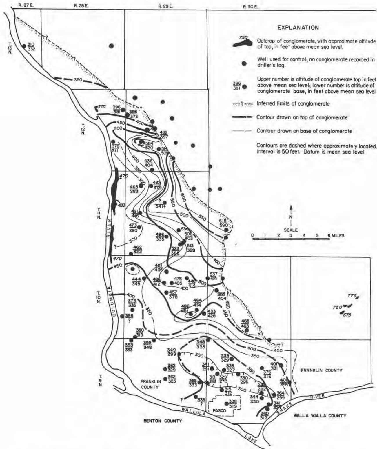
FIGURE 21.—Outcrops, subsurface extent, and structure of the Ringold conglomerate in southwestern Franklin County. (Interpretations based on drillers' lithologic logs.)
