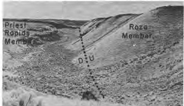
FIGURE 32.—View looking east along Spring Coulee, showing scarp of the Pinto Fault. (U.S. Bureau of Reclamation photo, 1949.)
