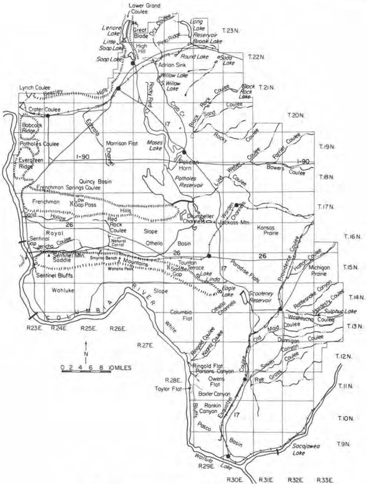
FIGURE 4.—Physiographic features of the project area.
