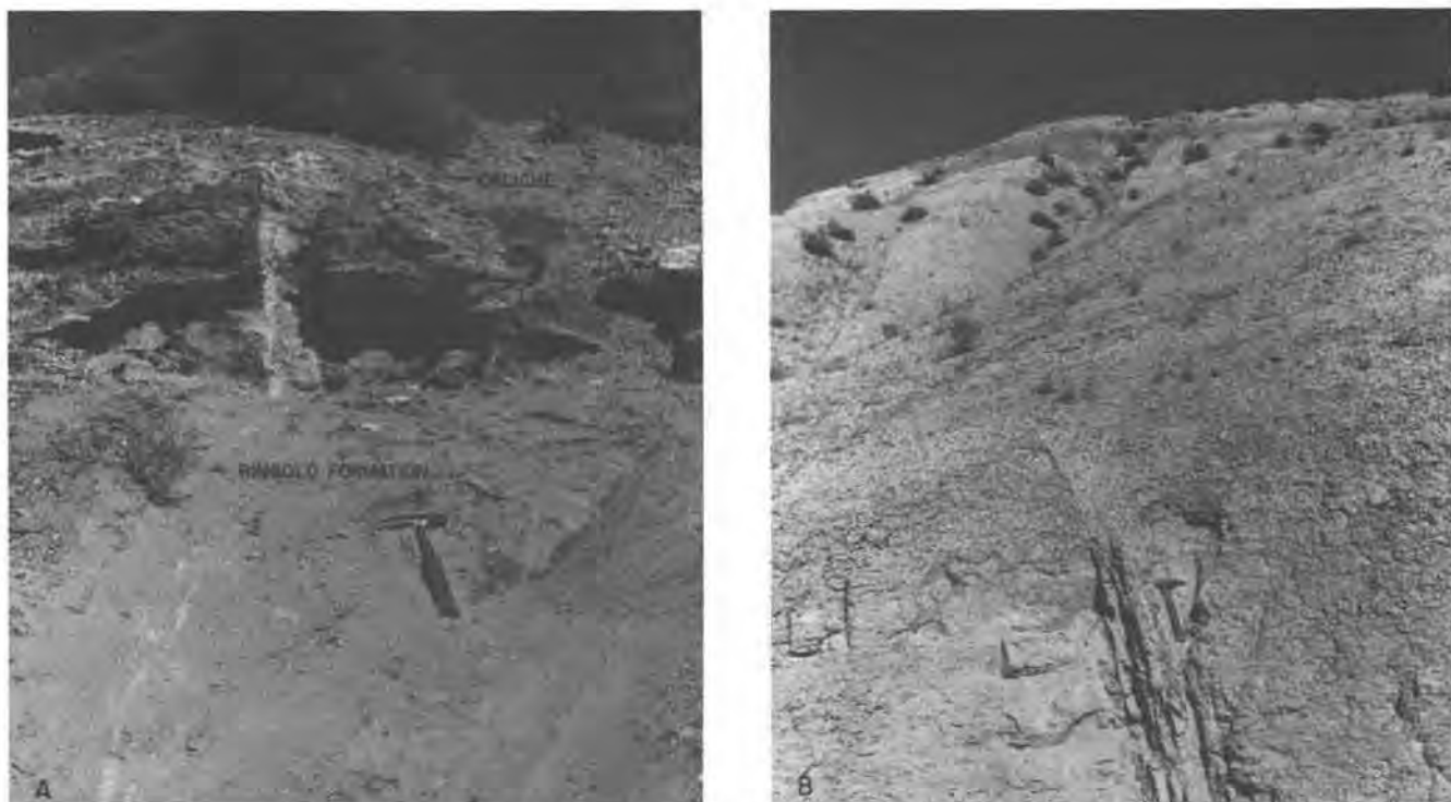
FIGURE 28.—Clastic dikes cutting through Ringold Formation and overlying caliche in SW \frac{1}{4} SW \frac{1}{4} sec. 3, T. 14 N., R. 26 E. A. Dike cutting caliche that caps Ringold Formation. B. Dike cutting Ringold laminated clay. Caliche capping shown in figure 28A is at top here, about 150 feet above hammer. (General Electric Hanford Operations photo.)
