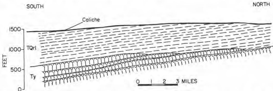
FIGURE 19.—Diagrammatic section showing the apparent regional unconformity due to offlap of individual basalt flows. Ty, Yakima Basalt, undifferentiated; TQrl, Ringold lacustrine clay and silt.
