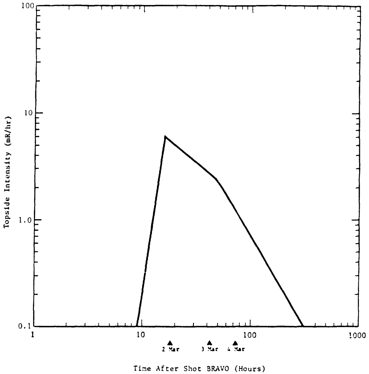
Figure 13. Estimated topside intensity on USS MOLALA (ATF-106) following Shot BRAVO.
