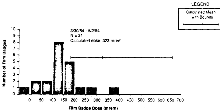
Figure 21. Film badge dosimetry for USS SHEA (DM-30).
