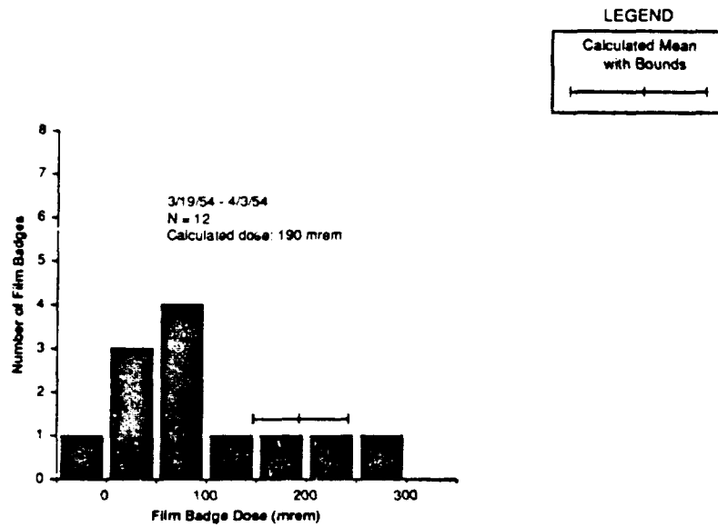
Figure 27. Film badge dosimetry for USS LST-1146.
