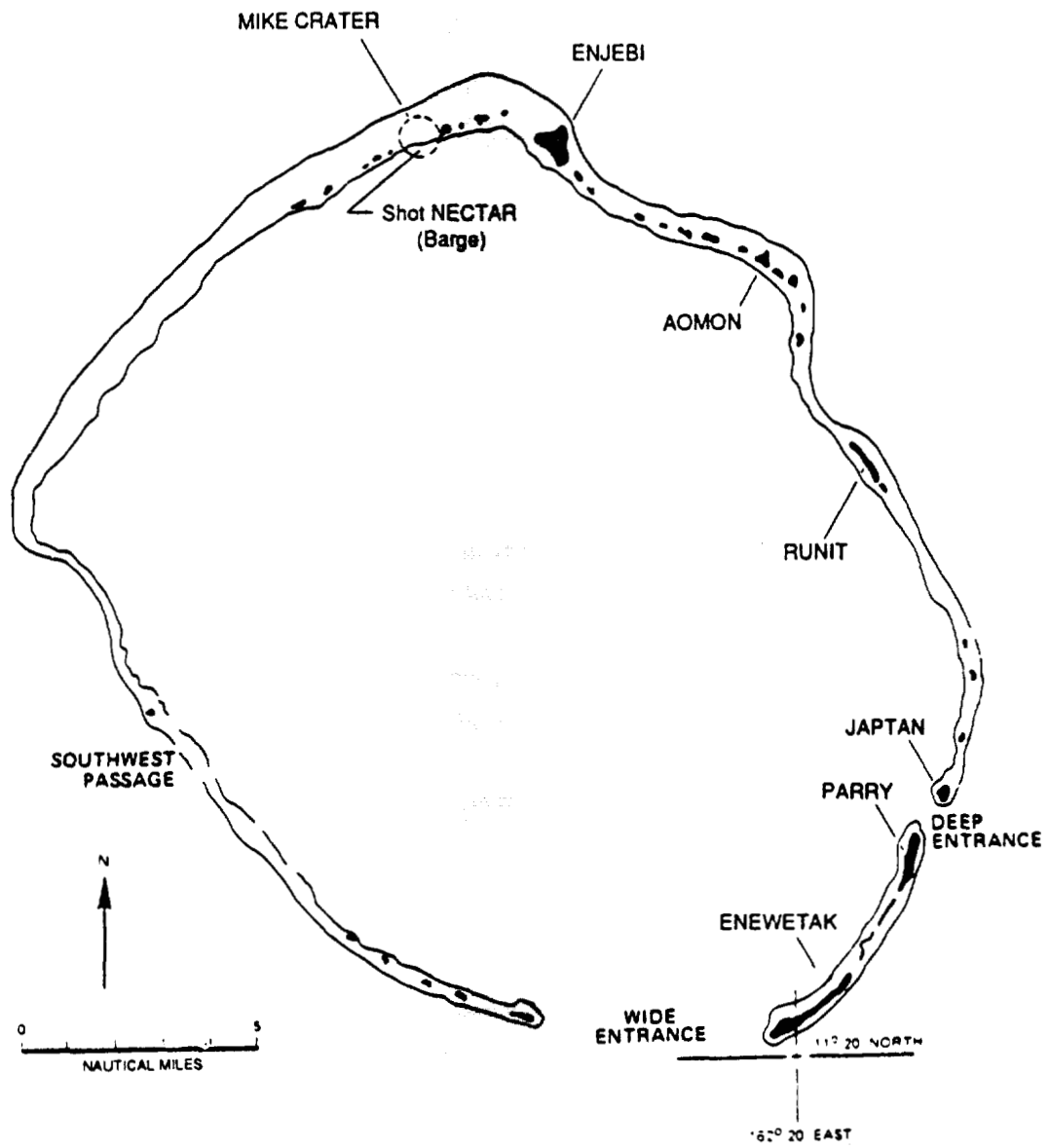
Figure 3. Enewetak Atoll, Operation CASTLE shot location.
