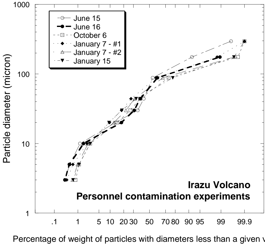
Figure 4-1. Cumulative weight distributions of volcanic ash particles in personnel contamination studies during eruption of Irazu Volcano in Costa Rica (Miller 1966b).
