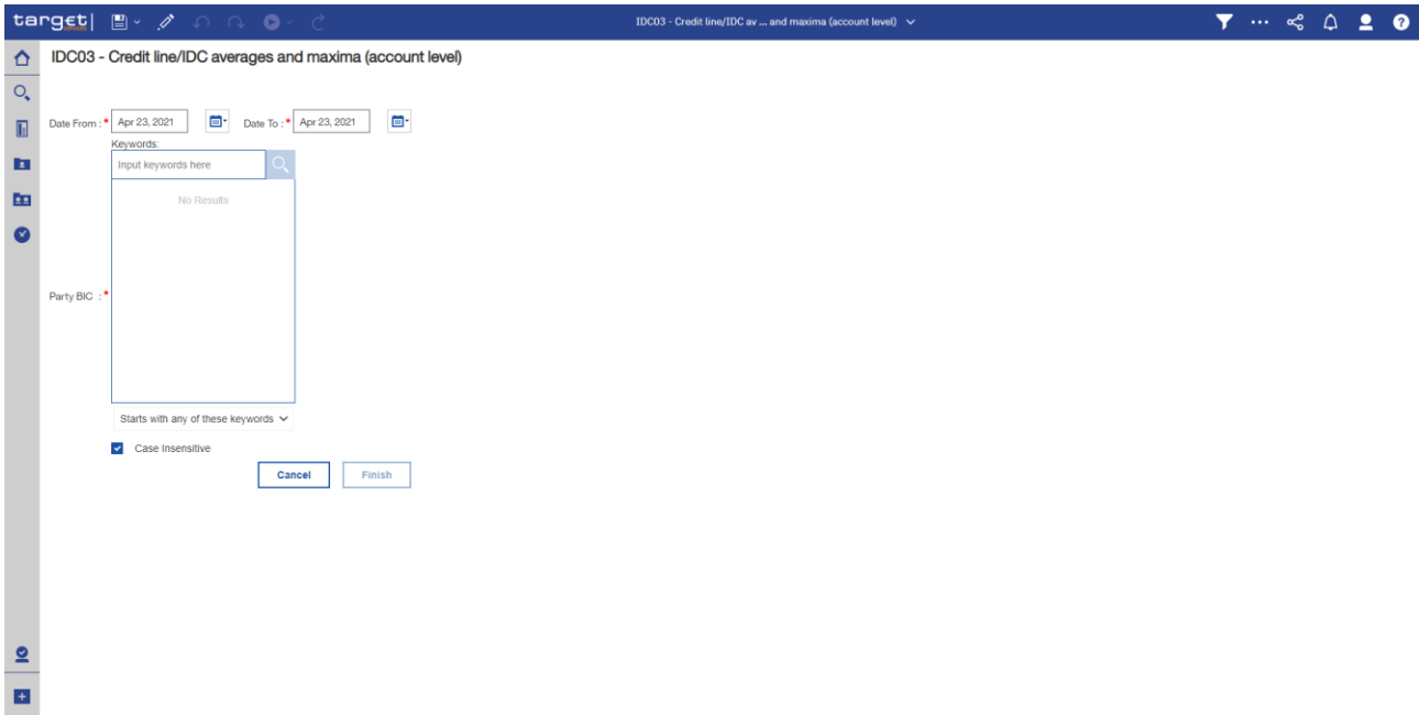
Figure 223 - IDC03 prompt
