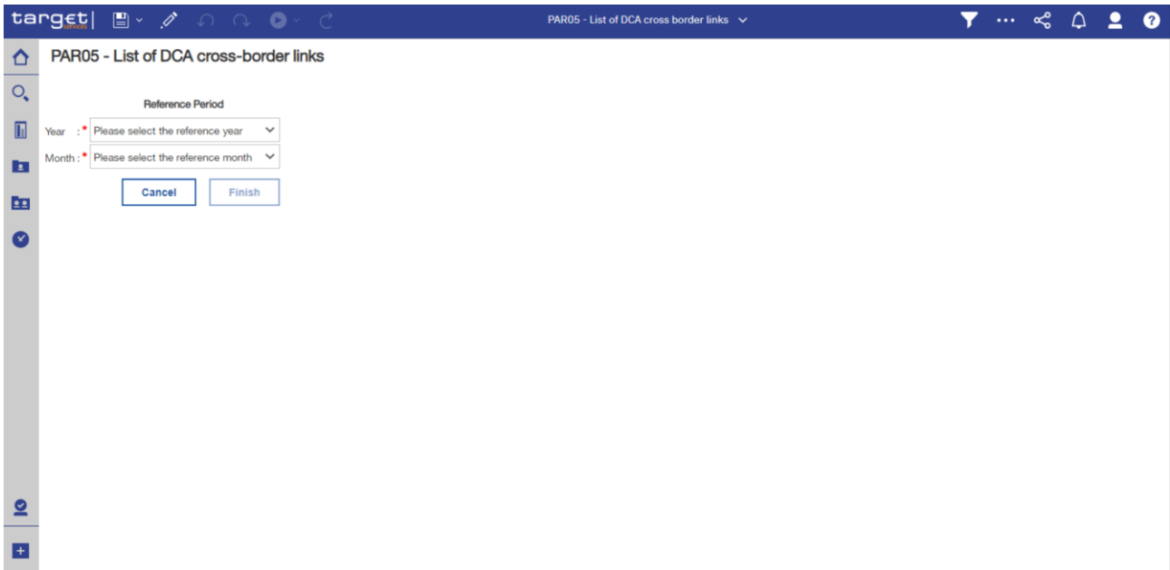
Figure 256 - PAR05 prompt
