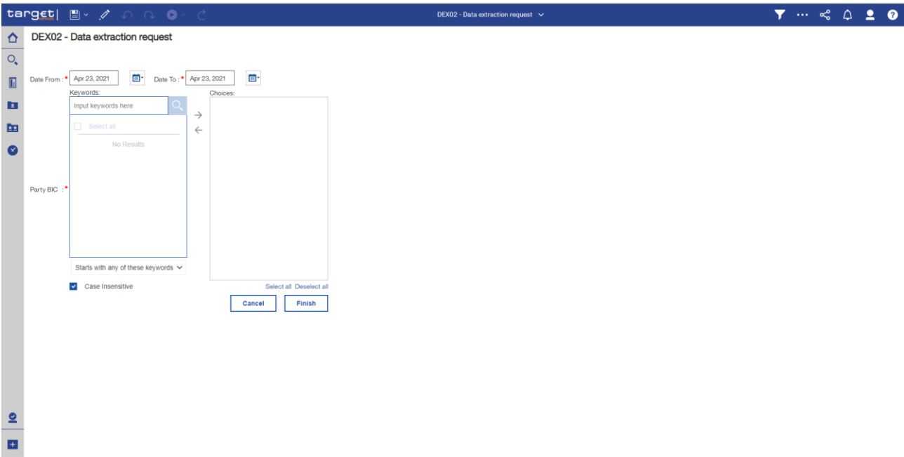
Figure 212 - DEX02 prompt{CR-111}
