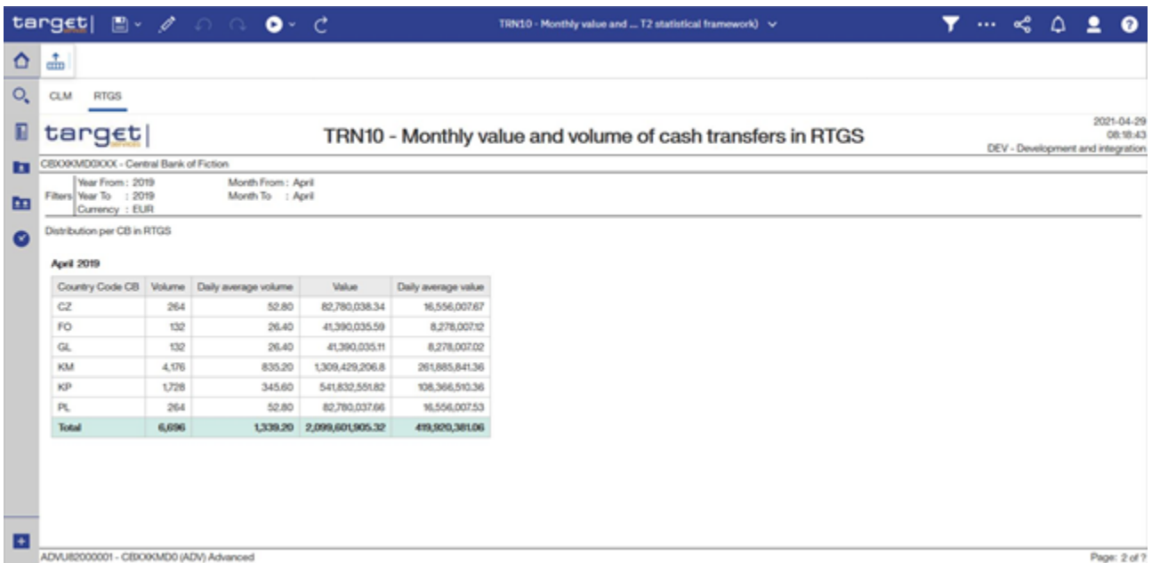
Figure 317 - TRN10 output (2)
