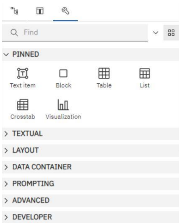
Figure 339 - Toolbox bar
