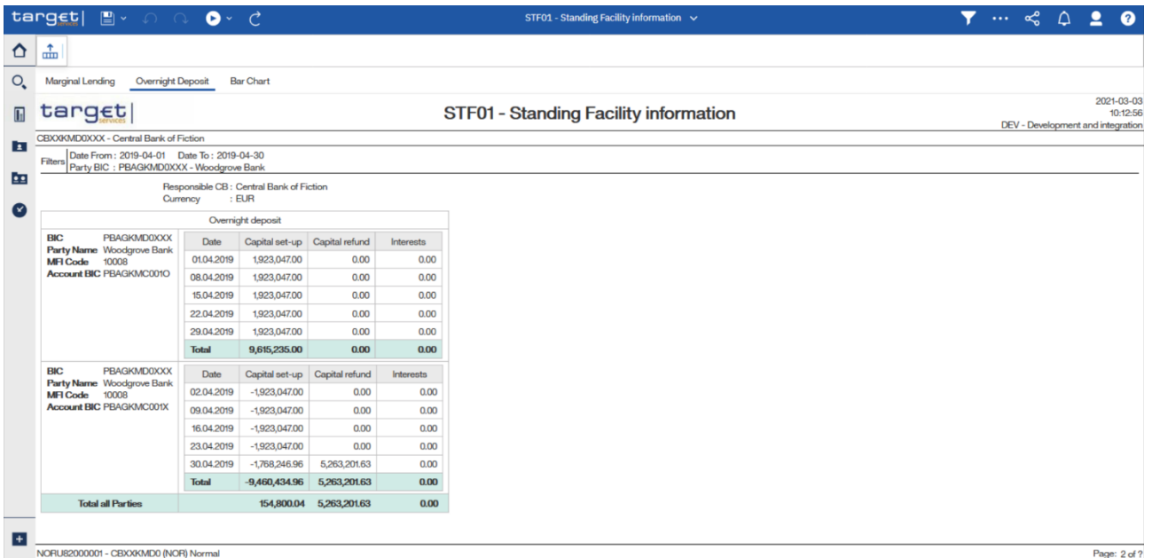
Figure 263 - STF01 output (2)
