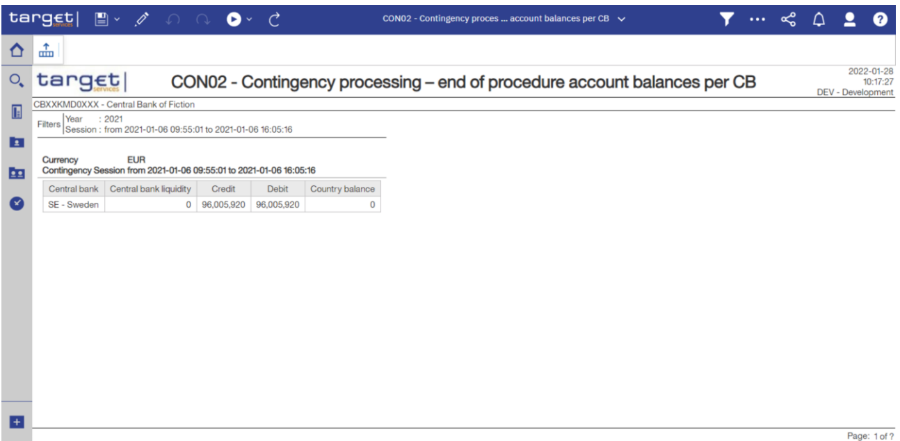
Figure 209 - CON02 output (2)
