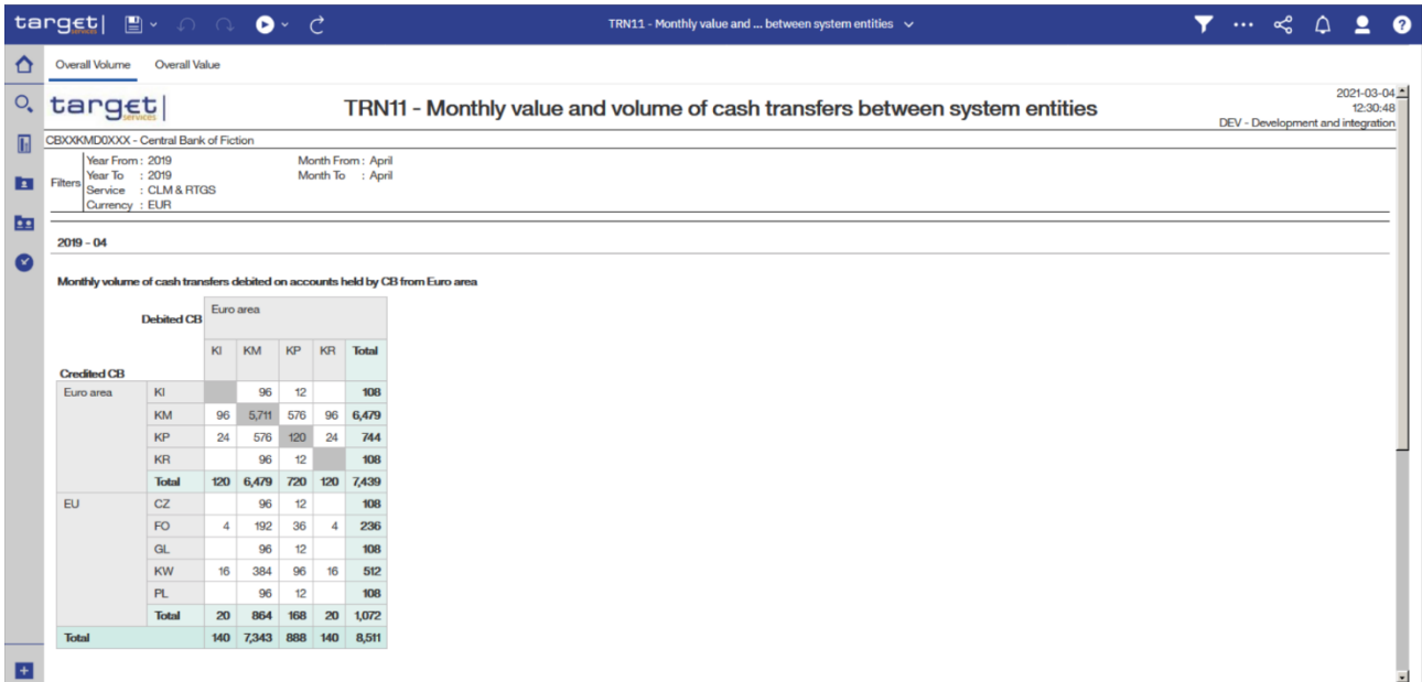
Figure 319 - TRN11 output (1)
