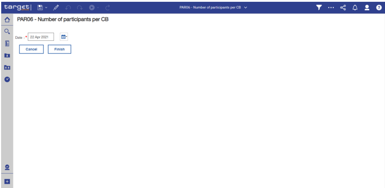
Figure 259 - PAR06 prompt
