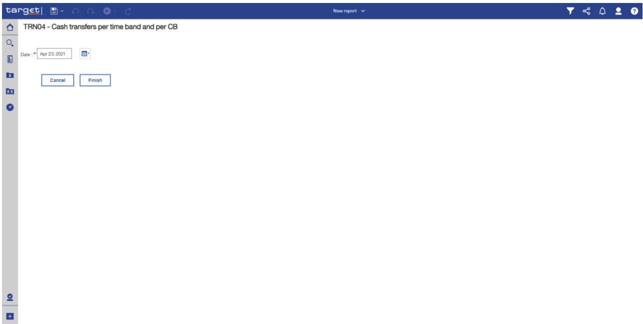
Figure 286 - TRN04 prompt
