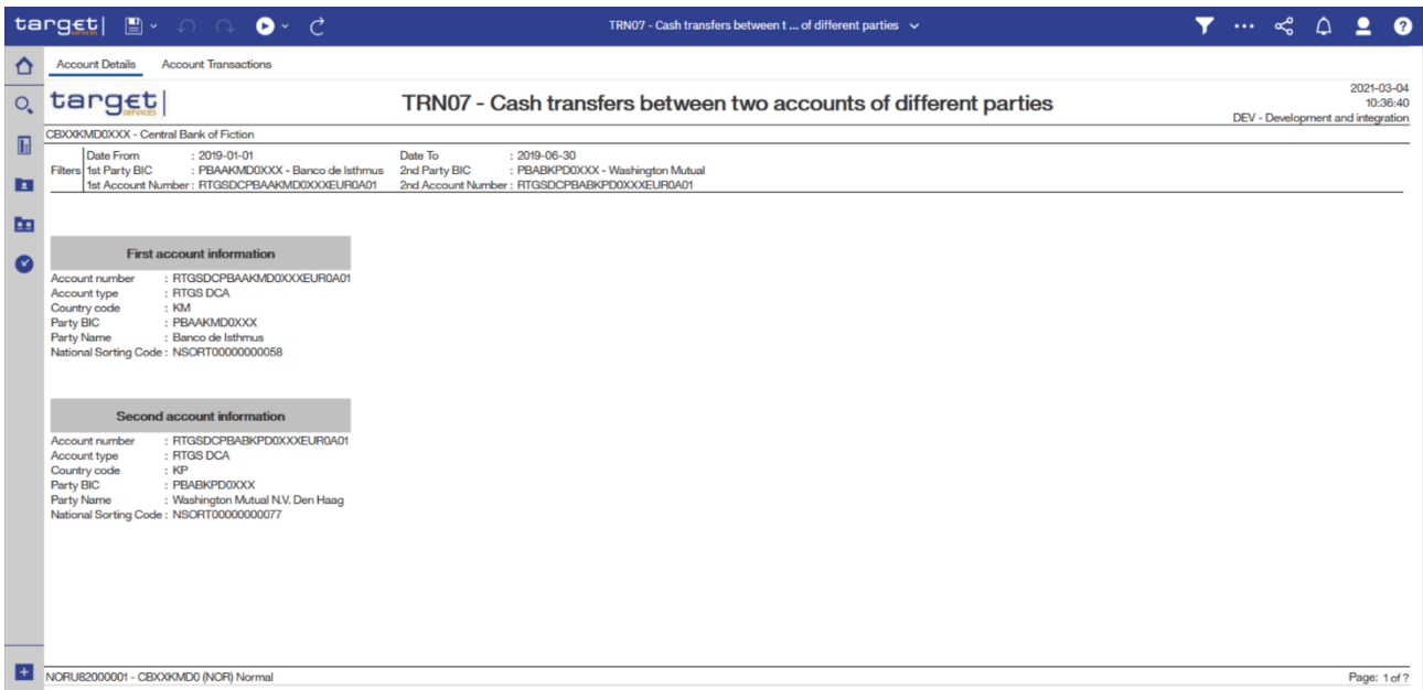
Figure 304 - TRN07 output (1)
