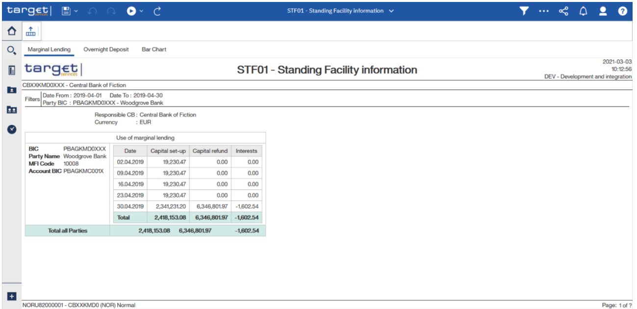
Figure 262 - STF01 output (1)
