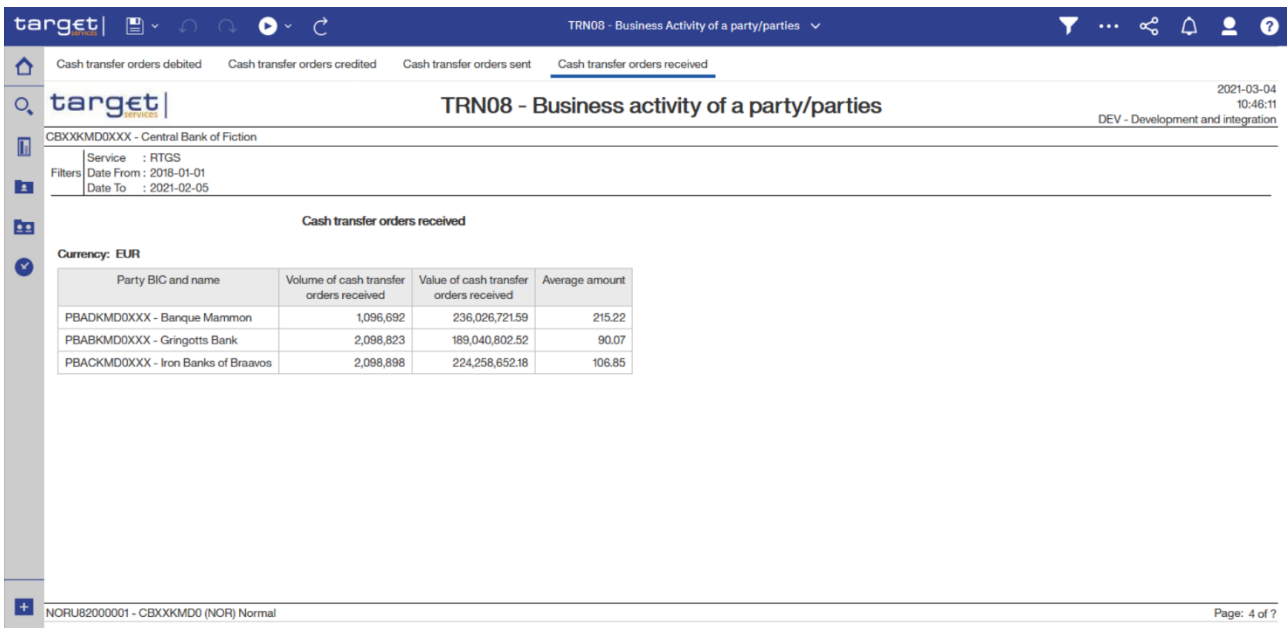
Figure 311 - TRN08 output (4)
