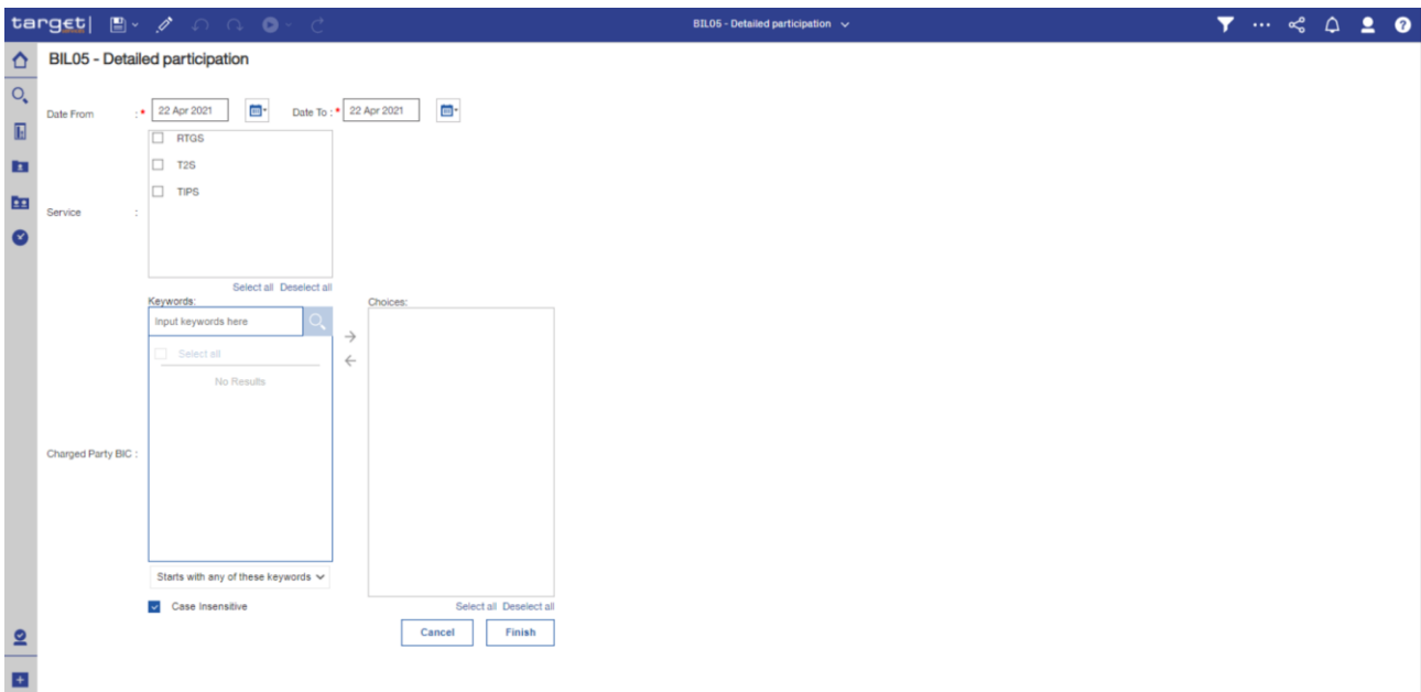
Figure 203 - BIL05 prompt
