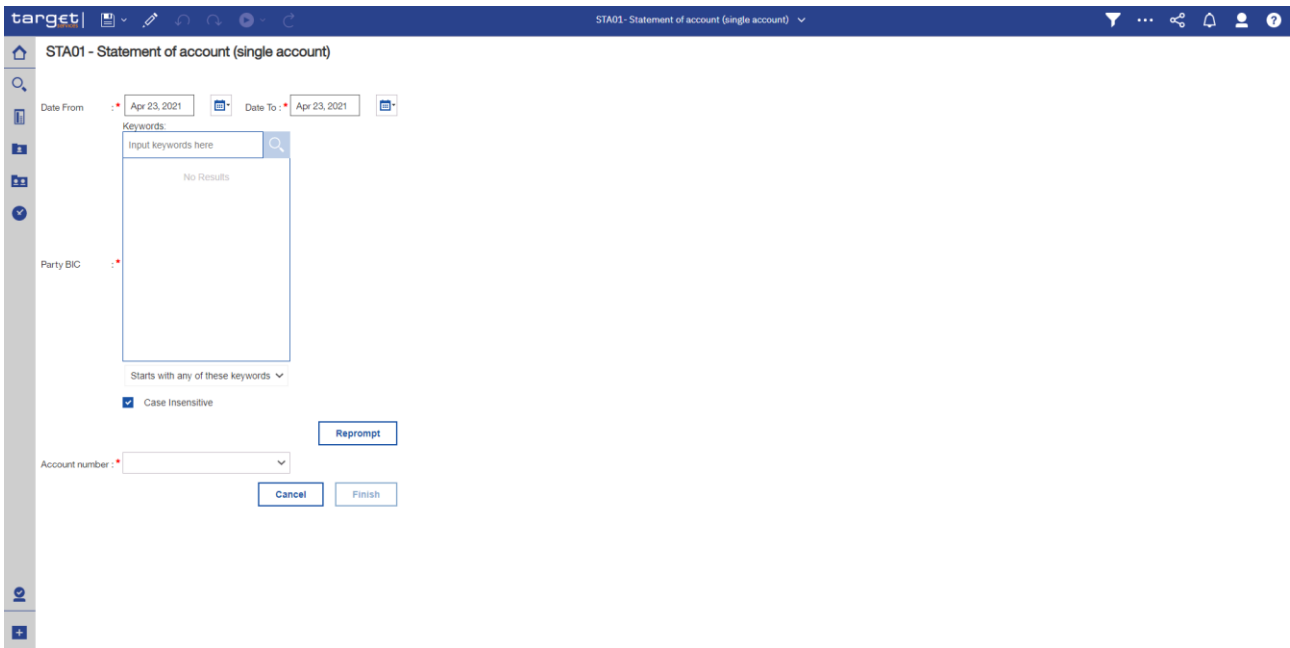
Figure 265 - STA01 prompt (1)
