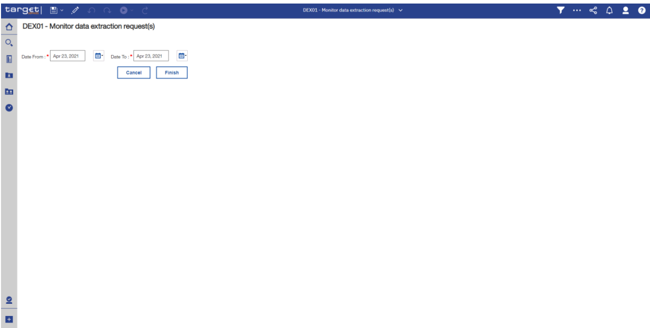
Figure 210 - DXE 01 prompt
