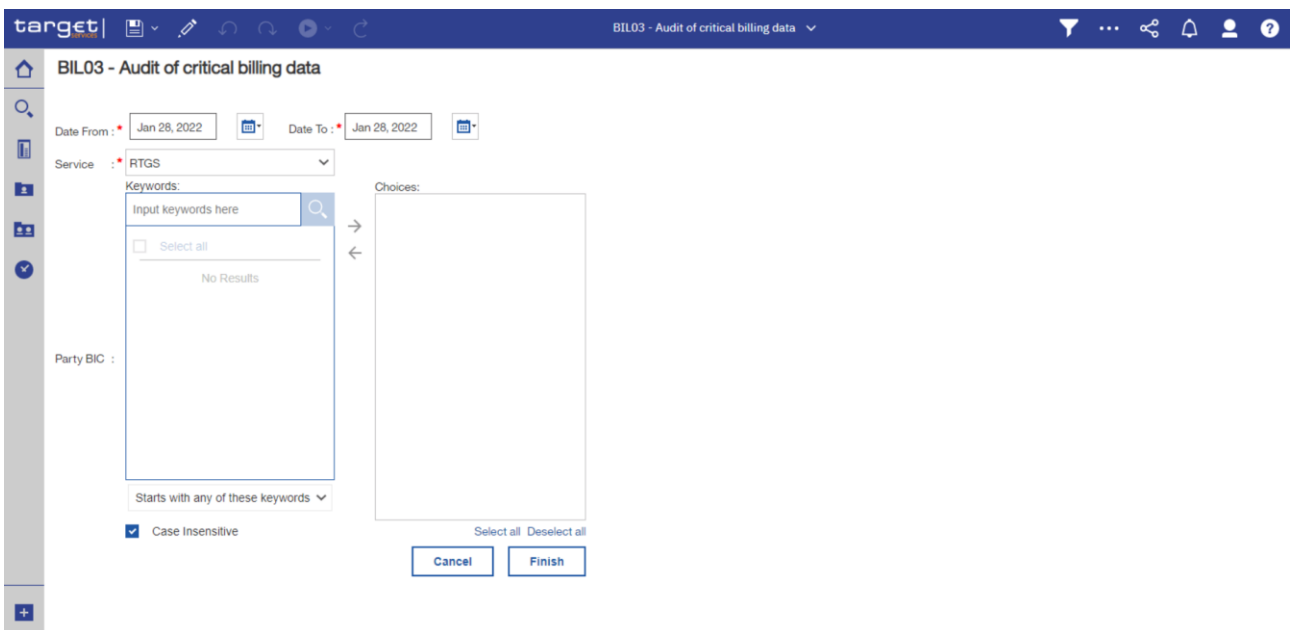
Figure 194 - BIL03 prompt
