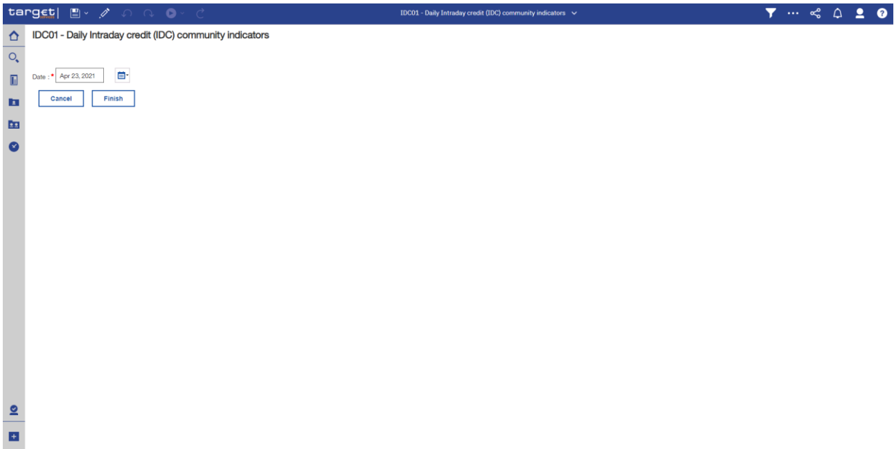
Figure 216 - IDC01 prompt
