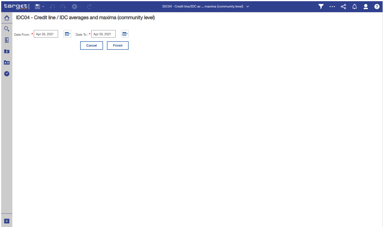
Figure 226 - IDC04 prompt
