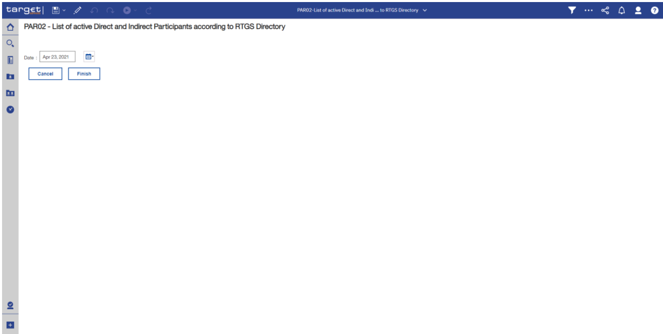
Figure 246 - PAR02 prompt
