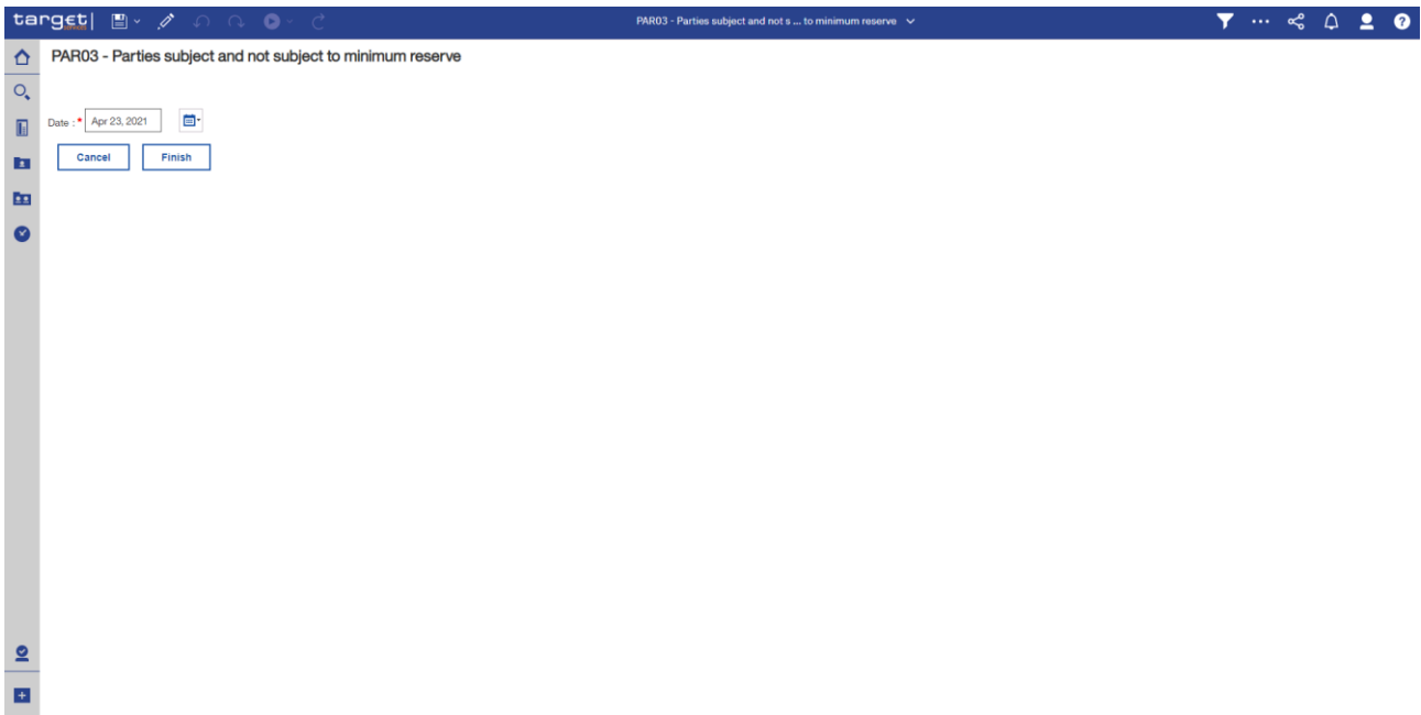
Figure 250 - PAR03 prompt
