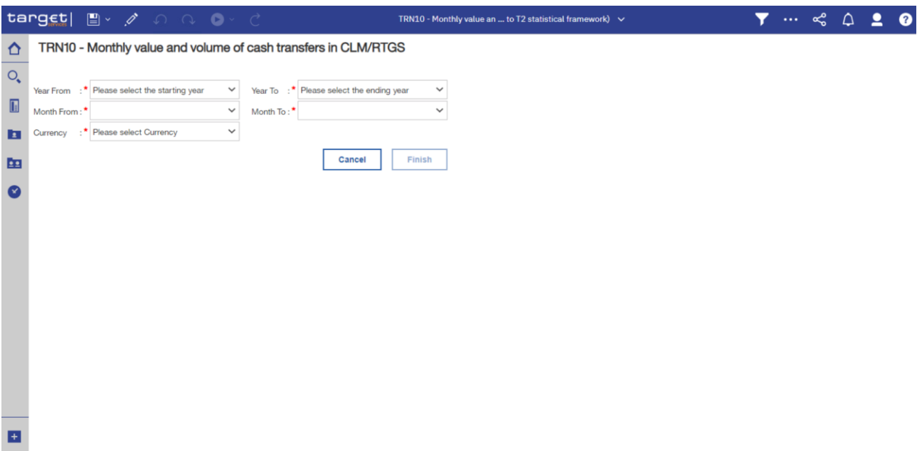
Figure 315 - TRN10 prompt
