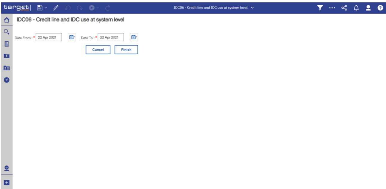
Figure 233 - IDC06 prompt
