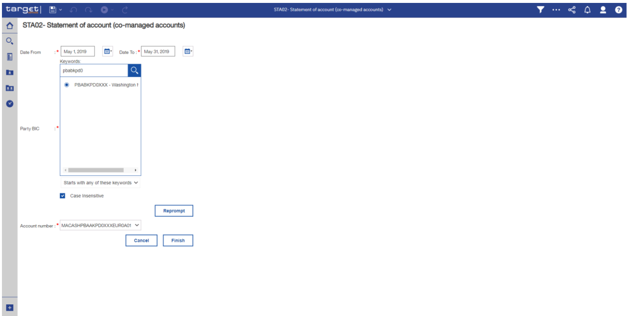
Figure 269 - STA02 prompt
