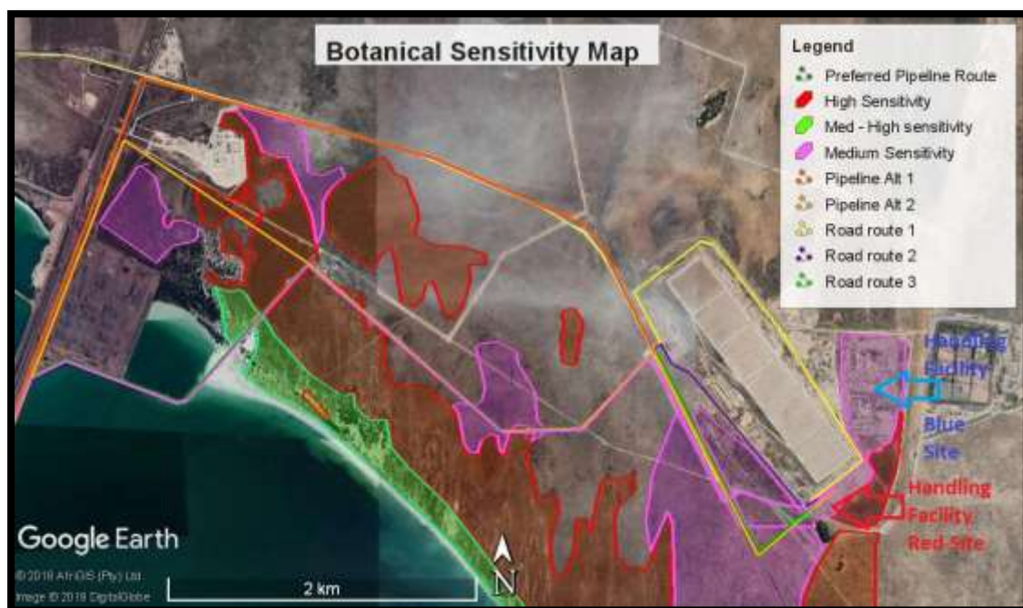
Figure 4: Map of the botanical sensitivity in the study area. Note that unshaded areas within the project area (generally within 50m of any infrastructure here assessed) are of Low sensitivity.
