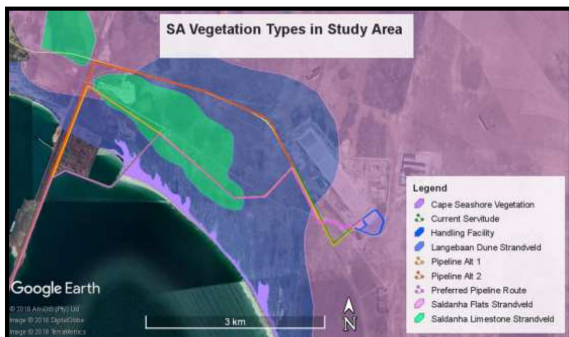
Figure 3: Extract of the SA Vegetation Map (Mucina & Rutherford 2012) showing the four vegetation types crossed by the various pipeline routes.
