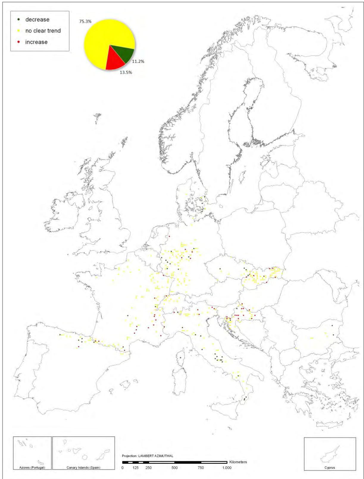
Figure 3-24: Development of mean plot defoliation (slope of linear regression) of Fagus sylvatica over the years 2002 – 2010
