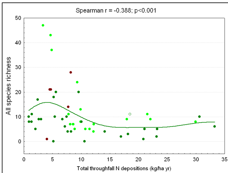
Figure 7-4: Biplot of the richness of all species as a function of the total throughfall nitrogen deposition at plot level. The fitting line is a distance weighted least square function with stiffness = 0.25. Plots (dots) are categorized according to the forest type: dark green: conifers; light green: deciduous broadleaves forests; brown: evergreen broadleaves forests; white: mixed forests.
