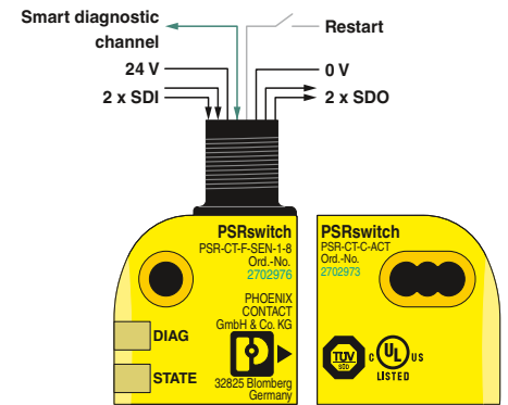
Smarter Sensor
