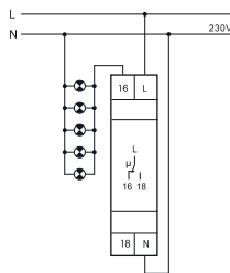
Direct control of the emergency light systems I \leq 16 A ⚡ Emergency light systems with own battery supply
