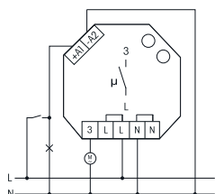
Fan control through light switch
