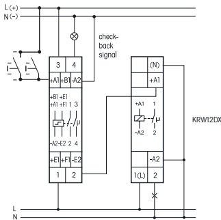
ES12Z with KRW12DX-UC
