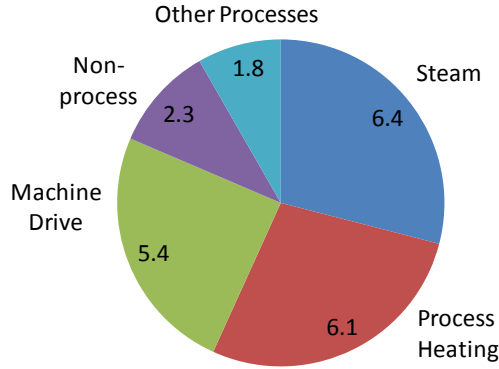
Figure 17. Industrial Primary Energy Use (Quads) Industrial primary energy use is dominated by thermal processes. Note: Approximately half of the energy required to generate steam use is additionally attributable to process heating energy demand. Source: Manufacturing Energy and Carbon Footprint Analysis on select energy-intensive industries, based on MECS data. Energy Information Administration. (2009). 2006 Manufacturing Energy Consumption Survey . Washington, DC: Department of Energy. Accessed at http://www.eia.gov/emeu/mecs/mecs2006/2006tables.html ; Industrial Technologies Program. (2011). Washington, DC: Department of Energy. Accessed at http://www1.eere.energy.gov/industry/rd/footprints.html
