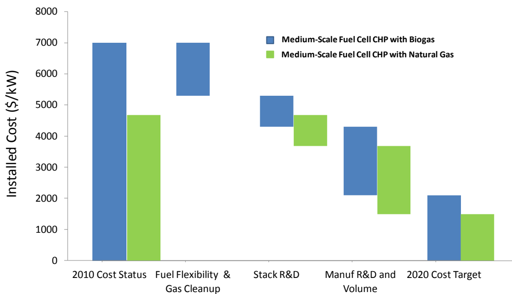
Figure 41. DOE Cost-Reduction Potential Through 2020. Analysis by the Department of Energy’s Fuel Cell Technologies Program. (2011). Washington, DC.
