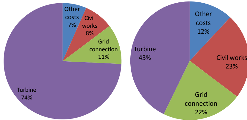
Figure 58. Capital Cost of Land-Based (left) and Offshore (right) Wind Power by Component Source: Wiser, R., et al. (2011). Chapter 7: Wind Energy. In IPCC Special Report on Renewable Energy Sources and Climate Change Mitigation . Page 66, Table 7.4. [O. Edenhofer, R. Pichs-Madruga, Y. Sokona, K. Seyboth, P. Matschoss, S. Kadner, T. Zwickel, P. Eickemeier, G. Hansen, S. Schlömer, C. von Stechow (eds)]. Cambridge, United Kingdom, and New York, NY, USA: Cambridge University Press. Accessed at http://srren.ipcc-wg3.de/report
