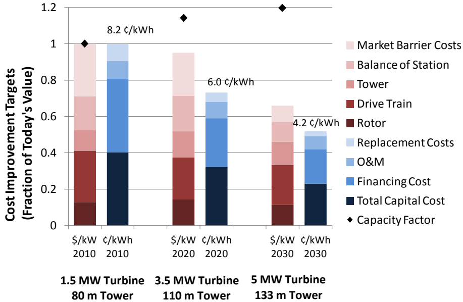
Figure 59. Potential Decrease in Land-Based Turbine Costs (red bars), LCOE (blue bars), and Associated Increase in Capacity Factor (black diamonds). 273, 274 Source: Internal Department of Energy Wind and Water Program Strategic Analysis, as part of roadmapping analysis.
