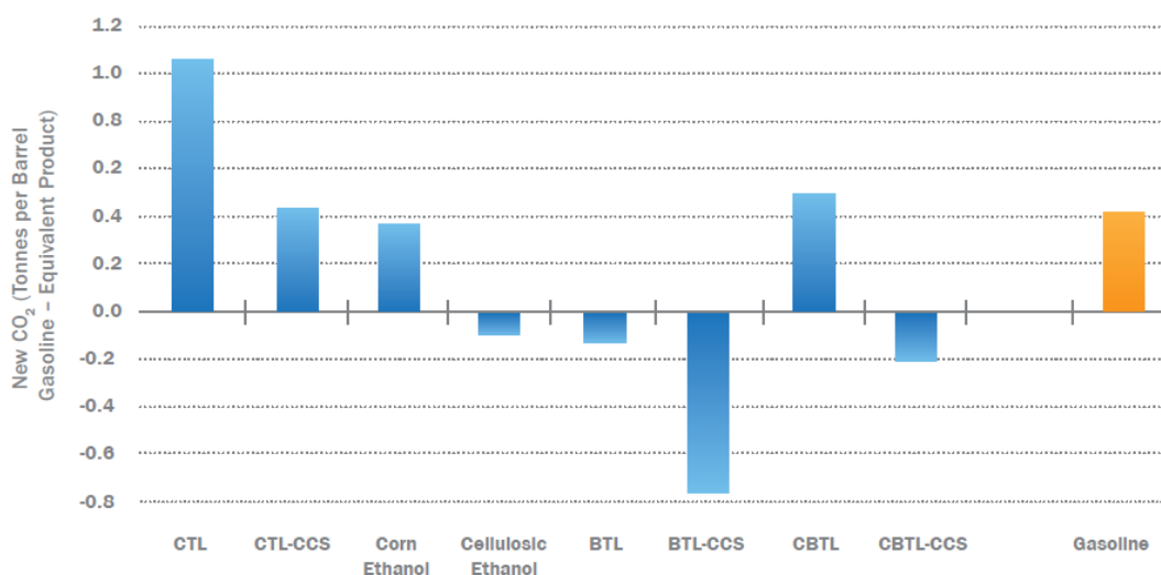
Figure 11. Lifecycle Carbon Emissions for Various Transportation Fuels The GHG emissions from some alternative fuels are less than those from conventional fuels, while others are higher. The production and extraction of feedstocks also have environmental impacts. CTL = coal-to-liquids, CCS = carbon capture and storage, BTL = biomass-to-liquids, CBTL = coal-and-biomass-to-liquids. There are many analyses for lifecycle carbon emissions from transportation fuels available, each with a unique perspective. This was adapted from America's Energy Future Panel on Alternative Liquid Transportation Fuels . (2009). p. 250. Washington, DC: National Academy of Sciences, National Academy of Engineering, National Research Council. Accessed at http://www.nap.edu/openbook.php?record_id=12620&page=250
