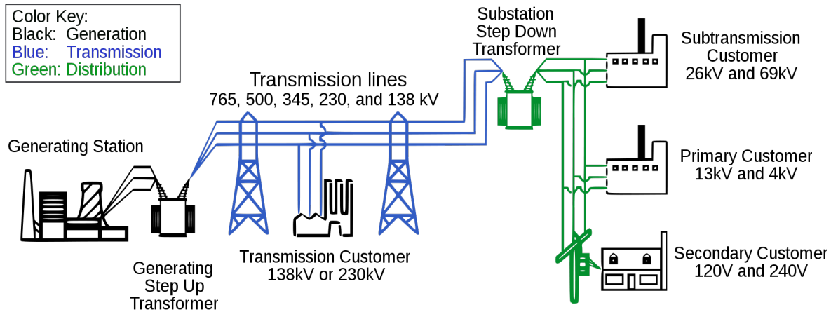
Figure 19. Simplified Schematic Showing Major Elements of the Electric Grid Source: U.S.–Canada Power System Outage Task Force. (2004). Final Report on the August 14, 2003 Blackout in the United States and Canada: Causes and Recommendations . Page 5. Accessed at http://www.ferc.gov/industries/electric/industryact/reliability/blackout/ch1-3.pdf
