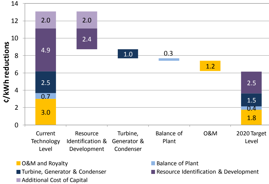
Figure 43. DOE Estimates of Cost Elements and Cost-Reduction Scenario for LCOE from Undiscovered Hydrothermal Resources The 2020 cost assumes the following reductions: Cost reduction of 50% in exploration and drilling, 50% in O&M, and 40% in power plant; one-year reduction from permitting time; and cost of capital reduction of 7% for all development stages (reduced from 15%–30% during resource identification and development). The reduction in upfront cost of capital is due to the reduction in the cost and risk of exploration. Source: Analysis by the Department of Energy’s Geothermal Technologies Program. (2011). Washington, DC.
