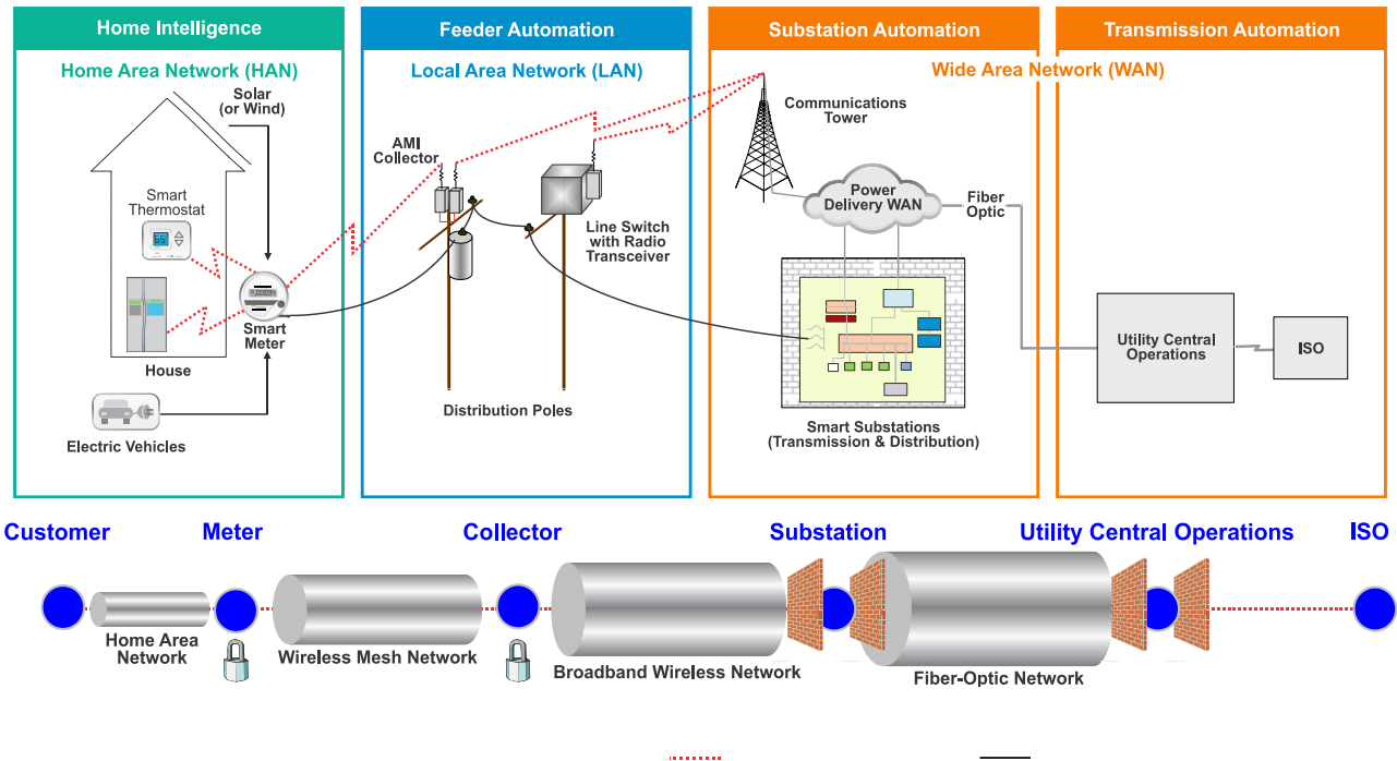
Figure 29. Representative Communications Architecture AMI = automated metering infrastructure, ISO = independent system operator.
