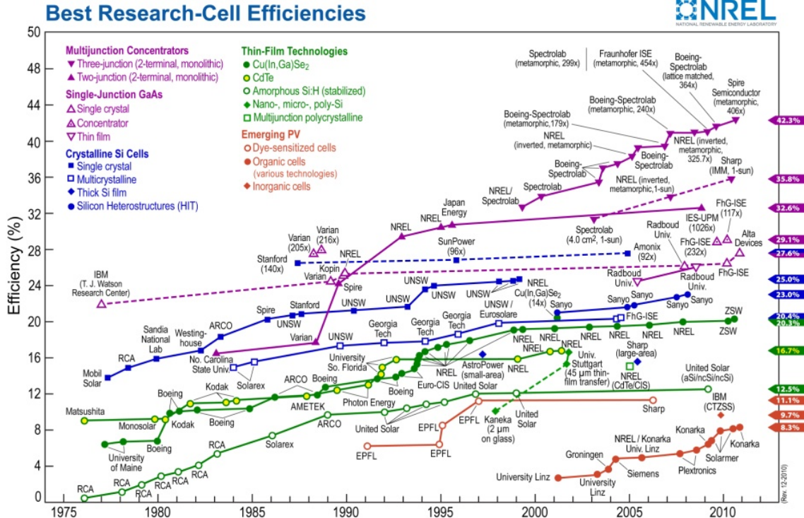
Figure 47. Best Research-Cell Efficiencies for PV Improvements in cell efficiencies driven by advancements in material science and semiconductor processing. The highest-efficiency research cell was achieved in 2010 in a multi-junction concentrator, at 42.3% efficiency. Source: National Renewable Energy Laboratory. (2011). Best Research-Cell Efficiencies . Golden, CO. Accessed at http://www.nrel.gov/ncpv/images/efficiency_chart.jpg
