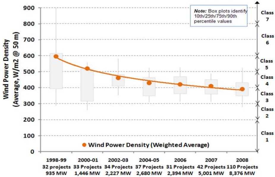
Figure 60. Wind Power Density of Installed Plants by Project Vintage Source: Wisner, R., and Bolinger, M. (2011). 2010 Wind Technologies Market Report . Page 39, Figure 21. Washington, DC: Department of Energy. Accessed at http://www1.eere.energy.gov/wind/pdfs/51783.pdf
