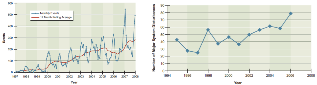
Figure 21. (Left) Transmission Loading Relief Events The number of transmission loading relief events is not an outage measure; it is the number of times a congestion limit is reached. Although this measure has been used to characterize transmission reliability, congestion limits can be reached purely for market reasons. (Right) Major Transmission System Disturbances Reported to North American Electric Reliability Corporation. Disturbances include electric service interruptions, unusual occurrences, demand and voltage reductions, public appeals, fuel supply problems, and acts of sabotage that can affect the reliability of the bulk electric systems. Source: Adapted with permission from The National Academies. (2009). America’s Energy Future: Technology and Transformation . Washington, DC: National Academies Press. Accessed at http://www.nap.edu/catalog/12091.html
