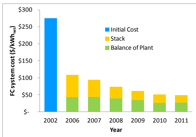
Figure 9. Modeled Fuel Cell System Cost at 500,000 Units (80 kW) per Year Modeled costs are based on an analysis of state-of-the-art components demonstrated at the laboratory scale and on projection to high-volume manufacturing. Source: Hydrogen and Fuel Cell Technologies Program. (2011). DOE Hydrogen Program Record: Fuel Cell Systems Cost—2011 . (Record #11012). Washington, DC: Department of Energy. Accessed at http://www.hydrogen.energy.gov/pdfs/11012_fuel_cell_system_cost.pdf
