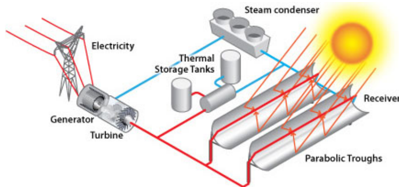
Figure 34. Parabolic Trough System Courtesy of: National Renewable Energy Laboratory. (1996). Linear Concentrator Solar Power Plant Illustration . Washington, DC: Department of Energy. Accessed at https://www.eeremultimedia.energy.gov/solar/graphics/linear_concentrator_solar_power_plant_illustration
