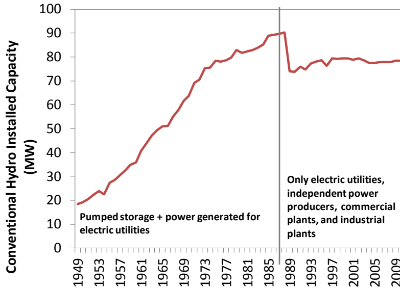
Figure 52. U.S. Installed Capacity of Conventional Hydropower, 1950–2010 Source: Energy Information Administration. (2011). Annual Energy Review 2011, Table 8.11a Electric Net Summer Capacity: Total (All Sectors), 1949-2010 . Washington DC: Department of Energy. Accessed at http://www.eia.gov/totalenergy/data/annual/showtext.cfm?t=ptb0811a
