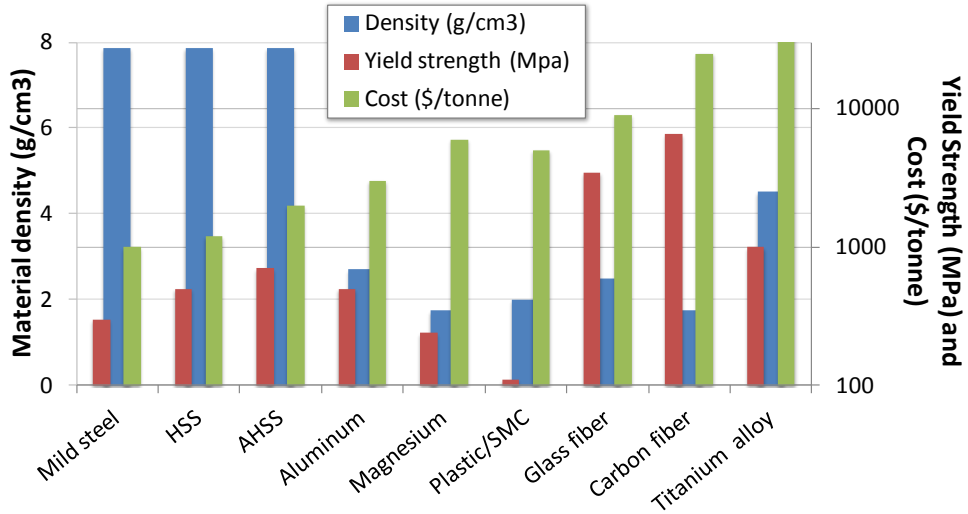
Figure 5. Materials Density, Strength, and Cost Adapted with permission from Lutsey, Nicholas P. (2010). Review of Technical Literature and Trends Related to Automobile Mass-Reduction Technology . (Research Report UCD-ITS-RR-10-10). Page 9, Figure 7. Davis, CA: Institute of Transportation Studies, University of California, Davis. Accessed at http://pubs.its.ucdavis.edu/publication_detail.php?id=1390
