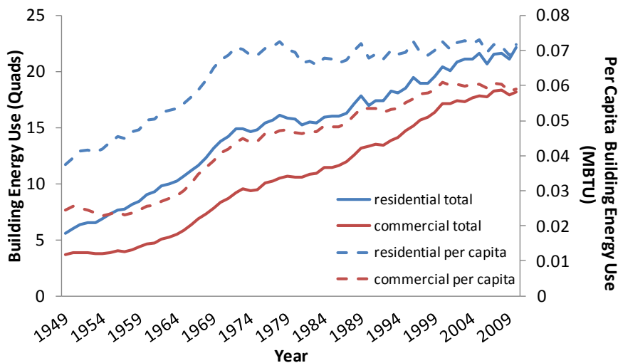
Figure 13. Residential (blue) and Commercial (red) Building Primary Energy Use (solid lines) and Per Capita Primary Energy Use (dotted lines) Since the 1950s Sources: Energy Information Administration. (2011).
