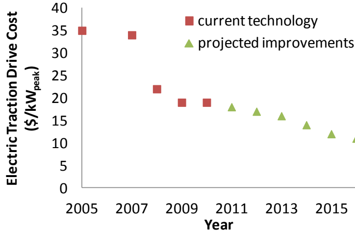
Figure 8. Electric Drive Cost This figure is a ground-up cost estimate based on proprietary data and cost models developed by an industry OEM.
