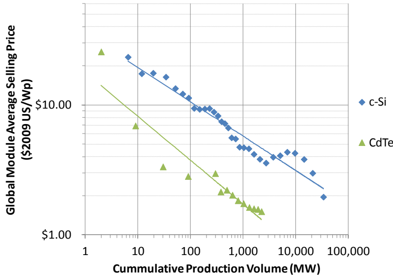
Figure 48. Solar PV Experience Curves Leading Technologies: Crystalline Silicon (c-Si), Cadmium Telluride (CdTe) Source: (CdTe) Sources: Adapted by the Department of Energy from (CdTe) First Solar Earnings Presentation, SEC Filings; (c-Si) Navigant, Bloomberg NEF, National Renewable Energy Laboratory internal cost models.
