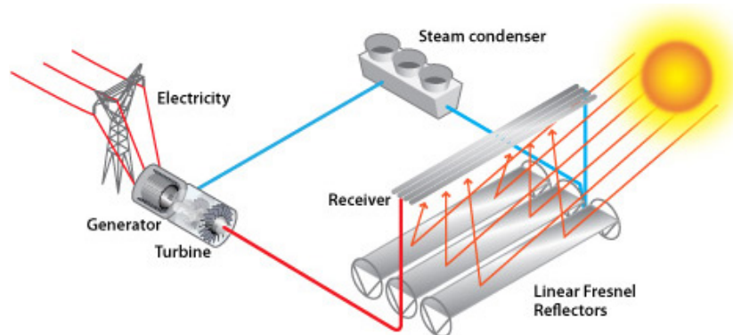
Figure 35. Linear Fresnel System Courtesy of: National Renewable Energy Laboratory. (2000). Linear Fresnel Power Plant Illustration . Washington, DC: Department of Energy. Accessed at https://www.eeremultimedia.energy.gov/solar/graphics/linear_fresnel_power_plant_illustration
