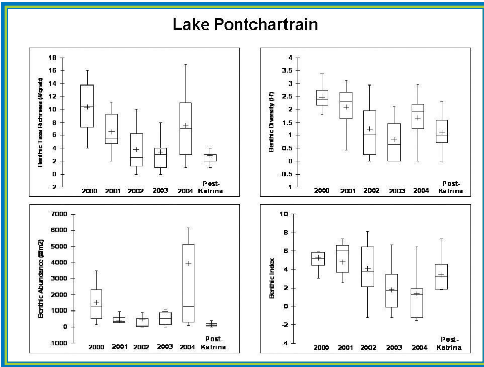
Fig. 4-4. Comparison of observed ranges in various benthic parameters in Lake Pontchartrain before (2000-2004) and after (2005) Hurricane Katrina. Boxes are inter-quartile ranges, horizontal lines within boxes are medians, plus marks are means, and whisker endpoints are 5th and 95th percentiles.
