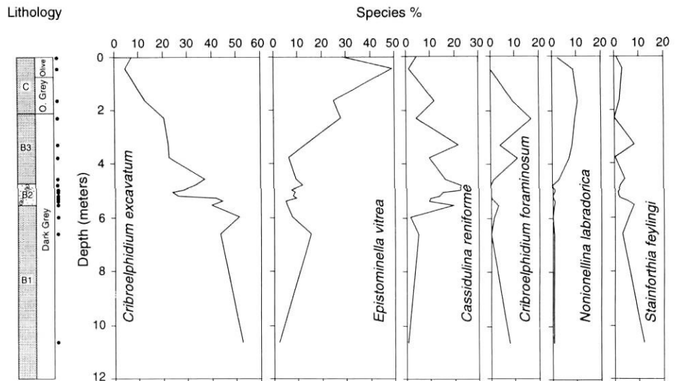
FIGURE 6. Stratigraphic section of core END 84B-08 showing lithology and distribution of key lithology and distribution of key indicator species. Dots beside stratigraphic column indicate sampled horizons (modified after Patterson, 1993).
