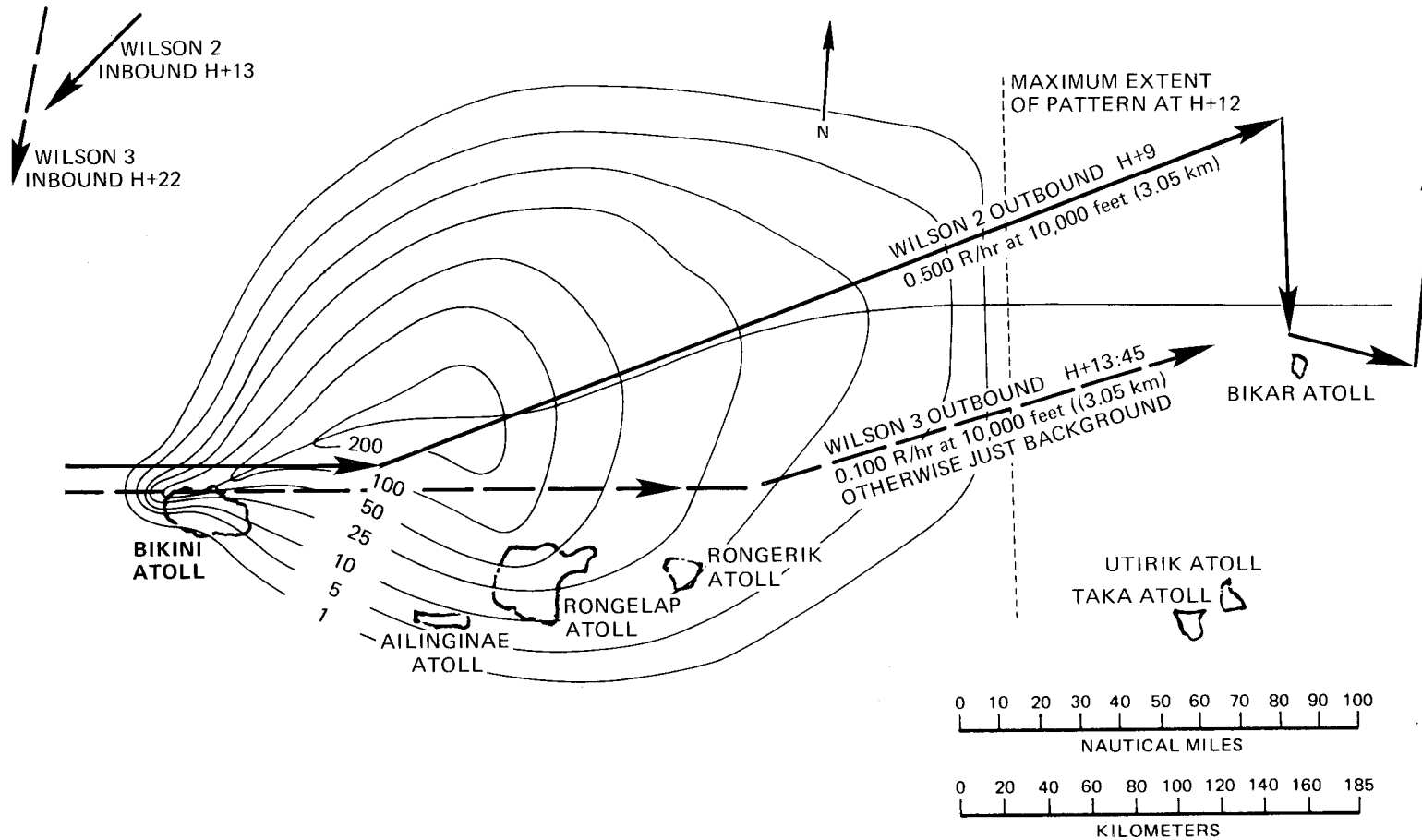
Figure 62. CASTLE, BRAVO reconstructed fallout at H+12; 1845 local time (R/hr). Reconstruction is by NRD and shows gamma field levels that would have existed had the fallout been on land areas (source: Reference 53).
