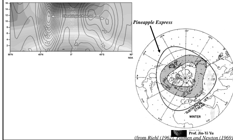
Vertical Cross Section of Temperature (°C) and Zonal Wind (m/s) at 180°E Longitude January Climatology NCEP/NCAR Reanalysis (1981-2010)
