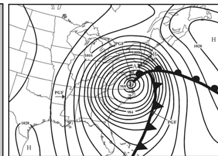
Extratropical Cyclone
