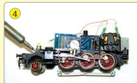
After a successful check connect the lighting cables. You may cut the cables of the adapter board as you please. Please make sure that the cables run properly!
