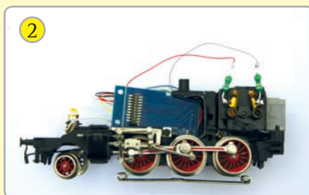
Install the 21MTC adapter board directly into the holding of the previous decoder. Mostly it can be easily plugged into the plastic holding.
