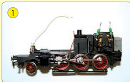
After adding the permanent magnet to the motor of your Delta® loco (as shown on the left page), remove the old Delta® decoder.
