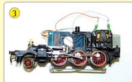
Plug the decoder onto the adapter board. At first wire the connections between the motor and the track. Leave the cables for lighting out for the time being and make your first driving test.
