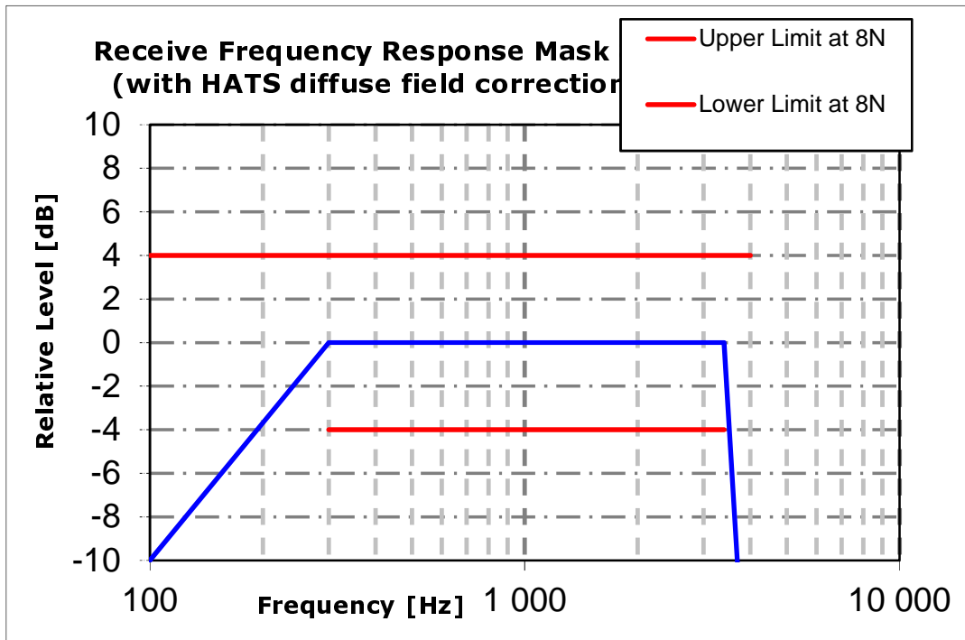
Figure 6.1.2-1: Receive frequency response mask for 8N application force
