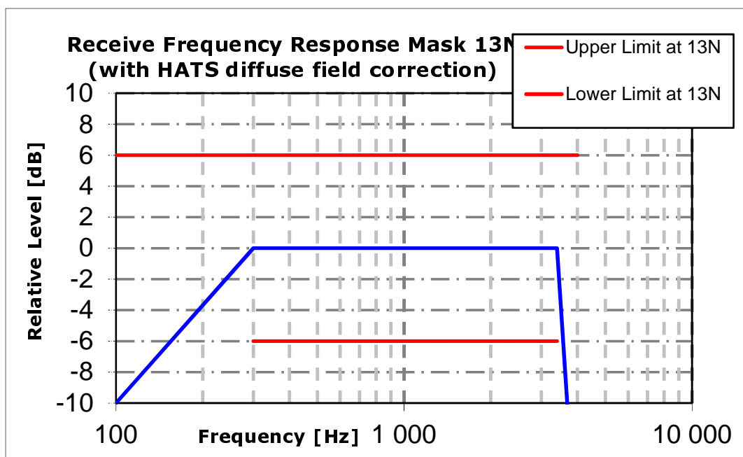
Figure 6.1.2-2: Receive frequency response mask for 13N application force
