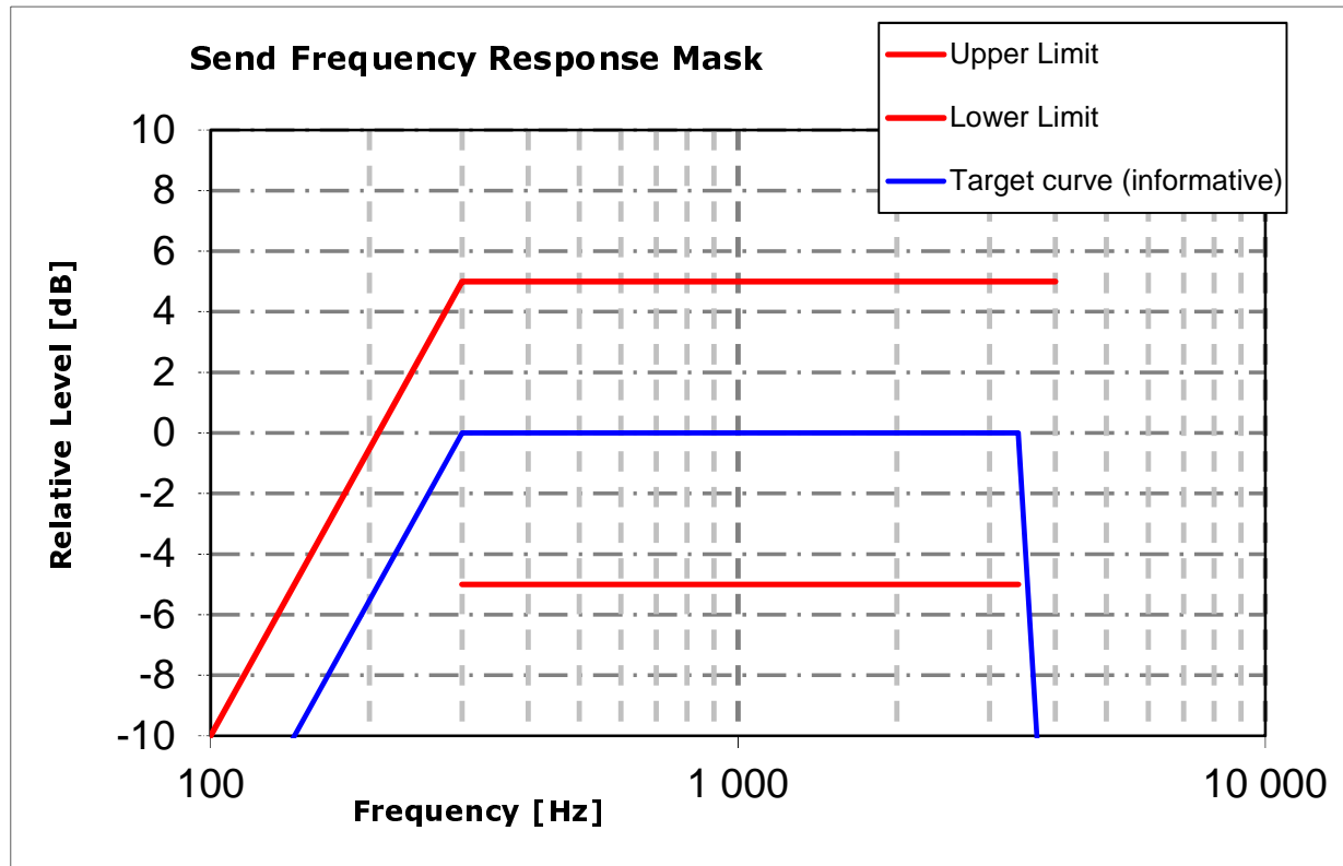
Figure 6.1.1-1: Send frequency response mask
