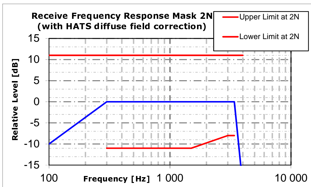
Figure 6.1.2-3: Receive frequency response mask for 2N application force
