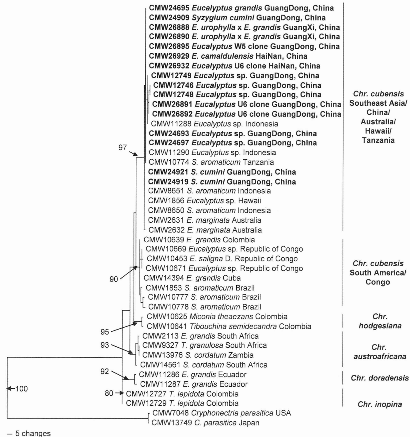
Fig. 4. One of 36 most parsimonious trees generated from combined sequence data of the internal transcribed spacer ribosomal DNA and \beta -tubulin gene sequence data and generated from heuristic searches performed on the combined data set (tree length of 348, CI of 0.937, and RI of 0.954). Bootstrap values (1,000 replicates) above 75% are indicated on the branches. Isolates sequenced in this study are in bold. Cryphonectria parasitica was used to root the tree.
