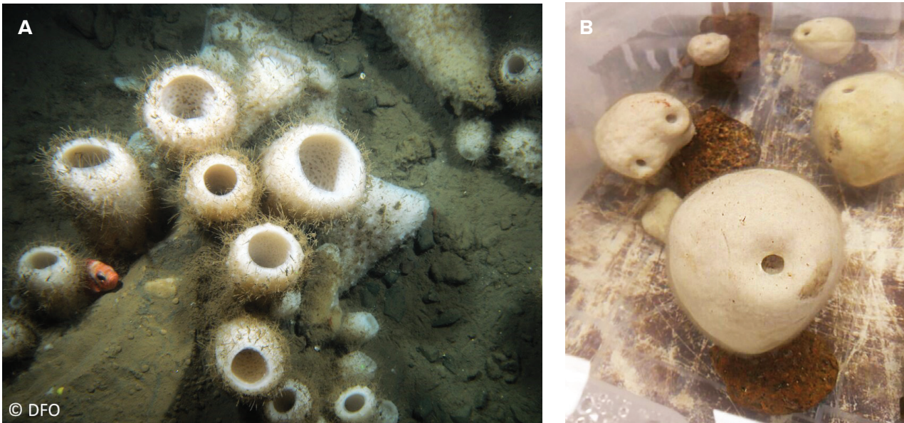
FIGURE 4 Examples of the sponge species used for sediment exposure experiments. A. The glass sponge Vazella pourtalesii . B. The demossponge Geodia barretti
