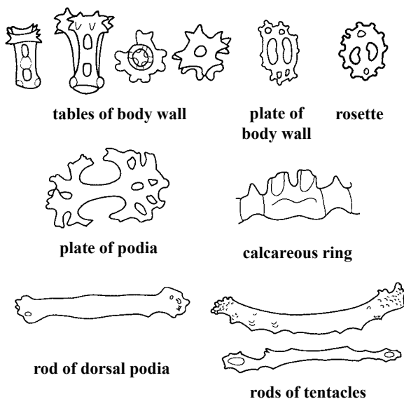
(after Cherbonnier, 1980)
