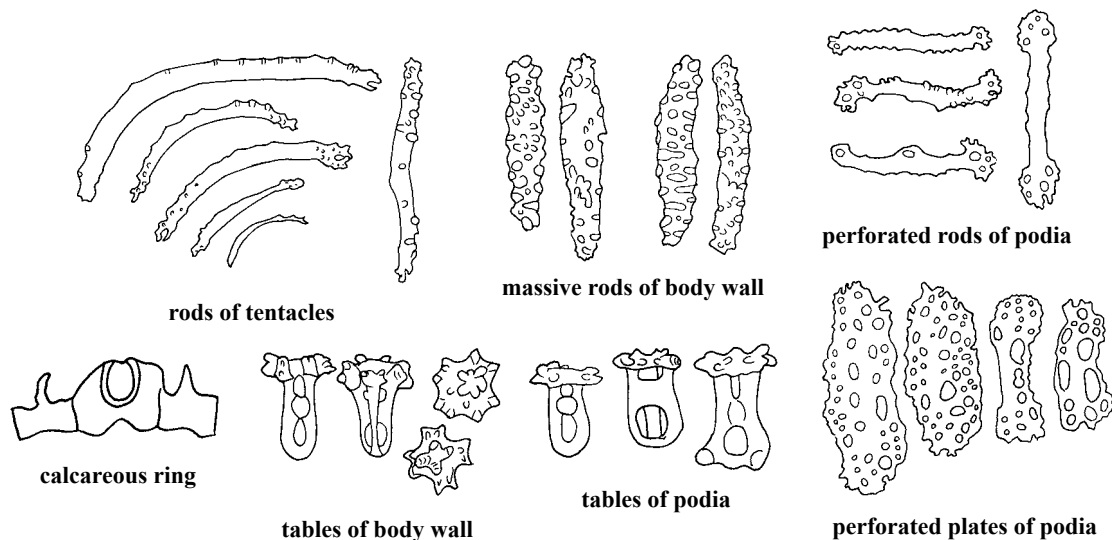
(after Massin, 1999)
