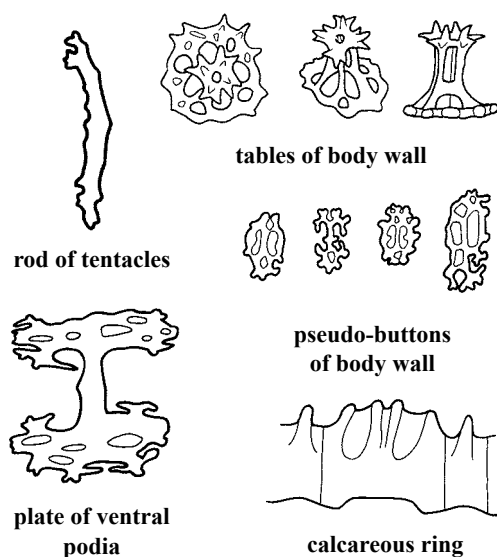
(after Cherbonnier, 1980)
