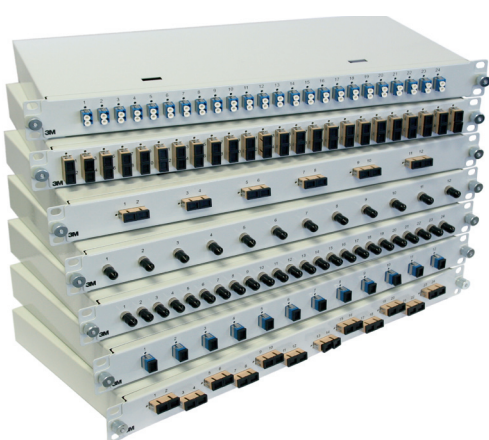
3M™ Eco SPP3 19" Fibre Optic Patch Panels
