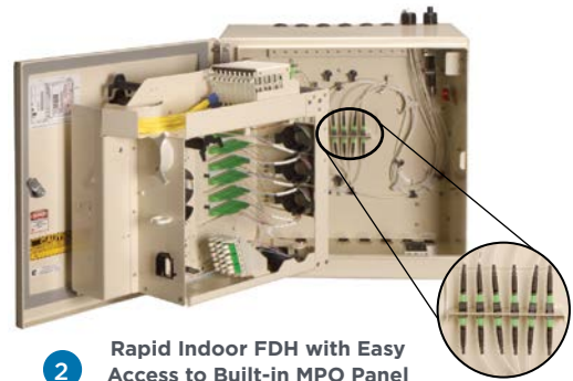
2 Rapid Indoor FDH with Easy Access to Built-in MPO Panel
