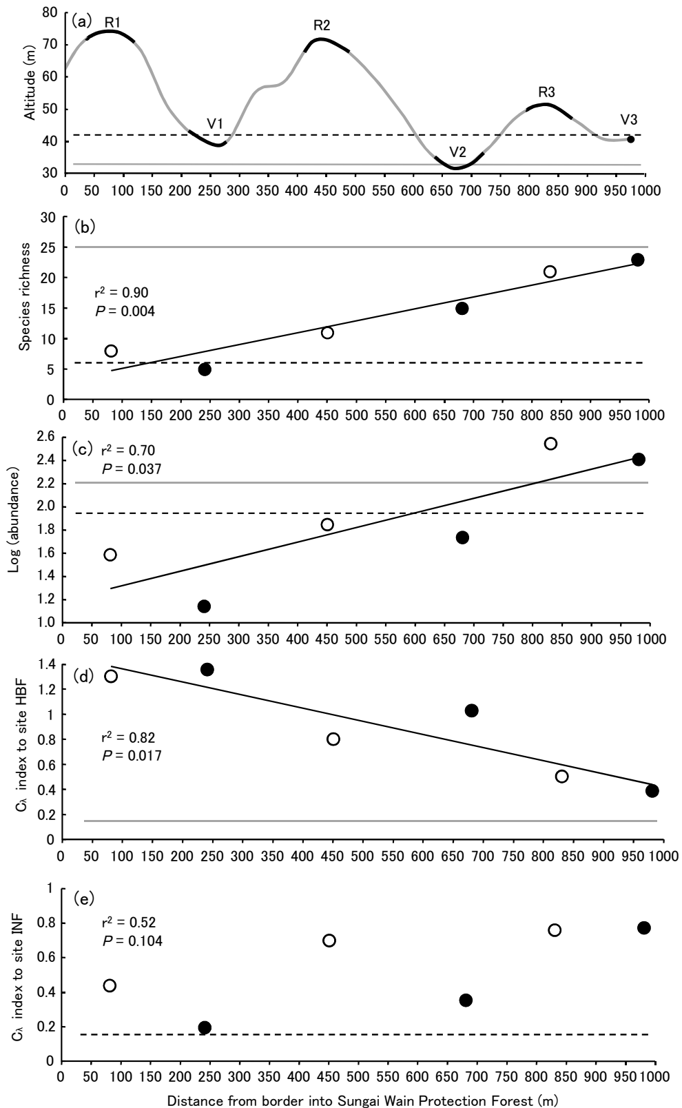
Fig. 2. Topography on the transect set in the study area (a) and species richness (b), the logarithm of abundance (number of beetle collected) (c), the Morisita's index of similarity ( C_{\lambda} ) to site HBF (d), and the Morisita's index of similarity ( C_{\lambda} ) to site INF (e) of the dung beetles collected at each site Topographies of trap transects were indicated with black lines in figure a. Data on control sites HBF and INF are shown as the dotted horizontal lines and the gray horizontal lines, respectively in figures. Closed circles and open circles indicate data in valley sites and data on ridge sites, respectively, and black lines in figures b, c, and d indicate data linear regression lines. Results of linear regression analyses are shown in figures b, c, d, and e.
