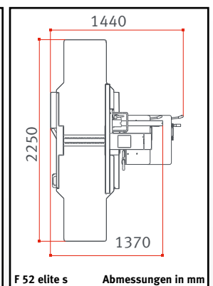
F 52 elite s Abmessungen in mm
