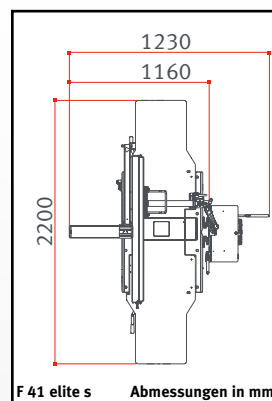
F 41 elite s Abmessungen in mm
