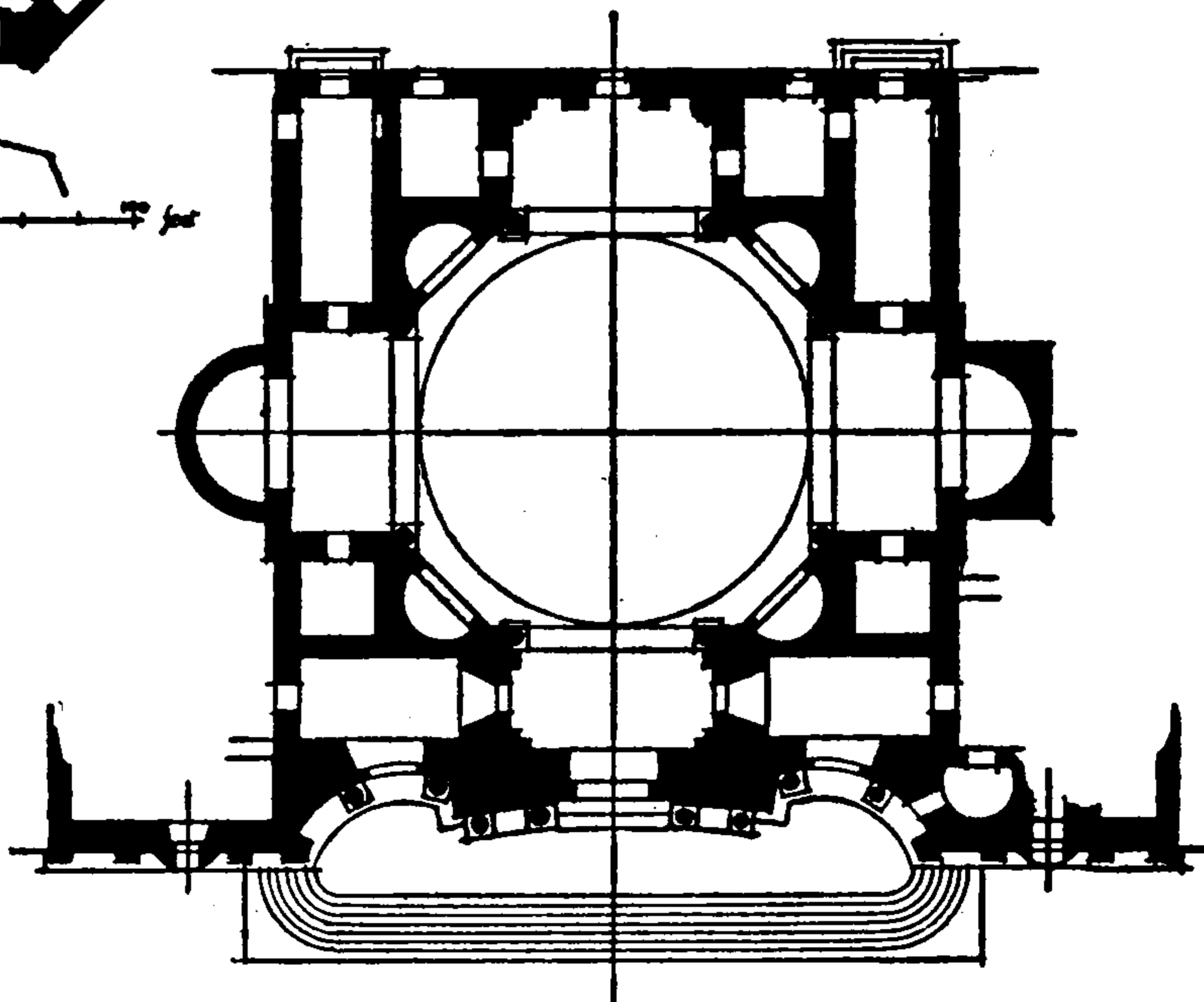
Figs. 7, 8, 9.—Plans of Roman Churches.
