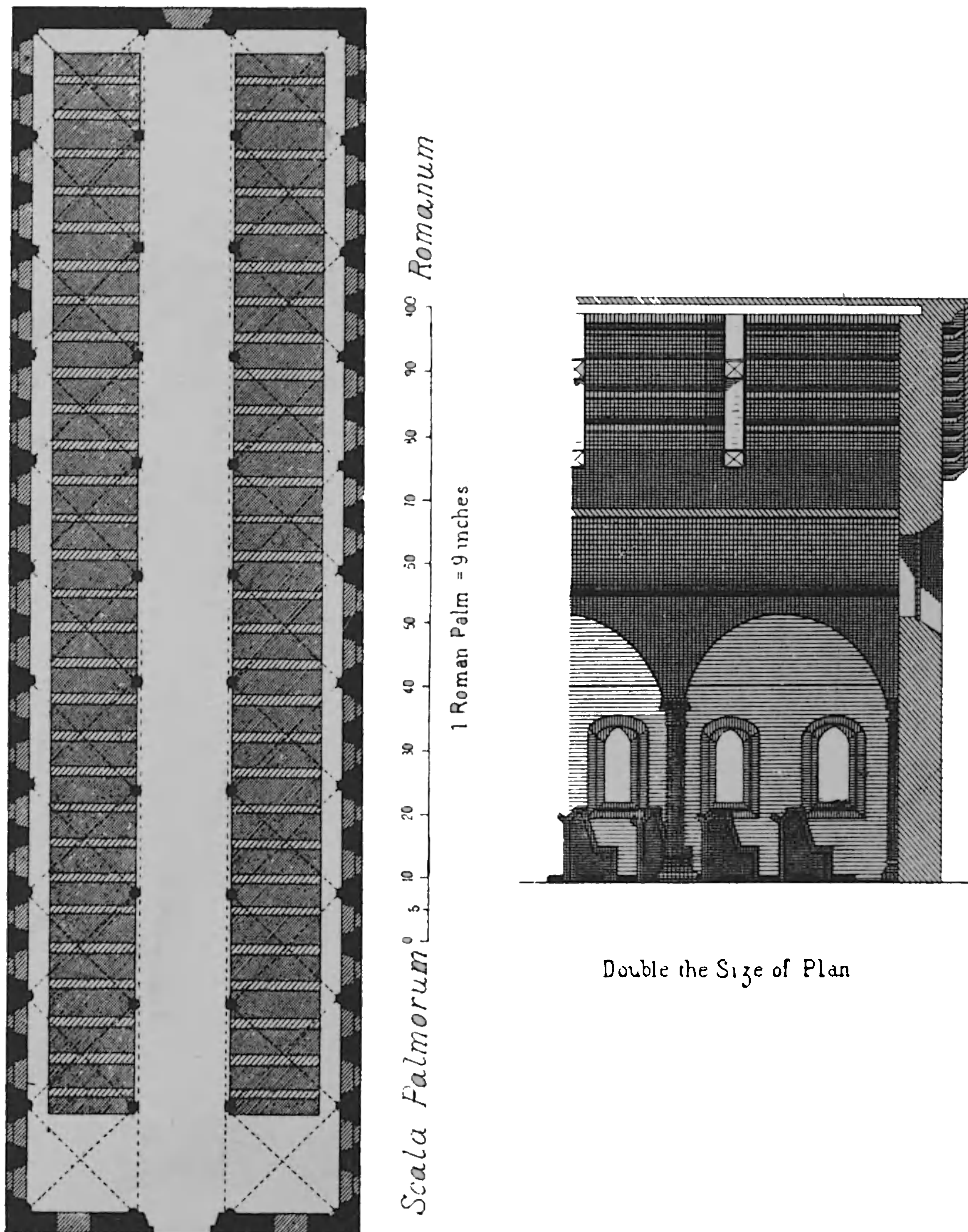
Figs. 90, 91. Ground-plan and section of Library at Cesena.
