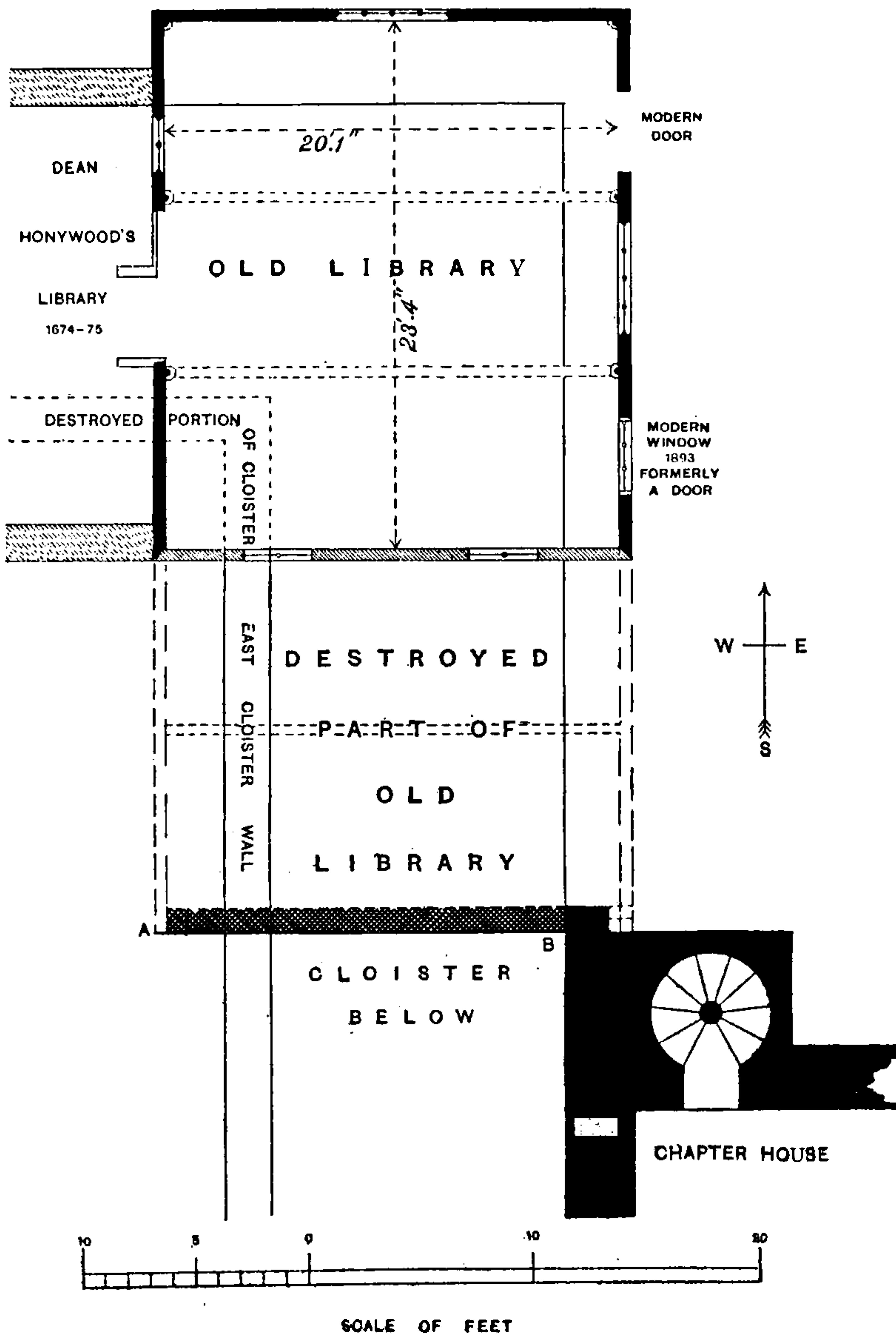
Fig. 38. Plan of the Old Library, Lincoln Cathedral.
