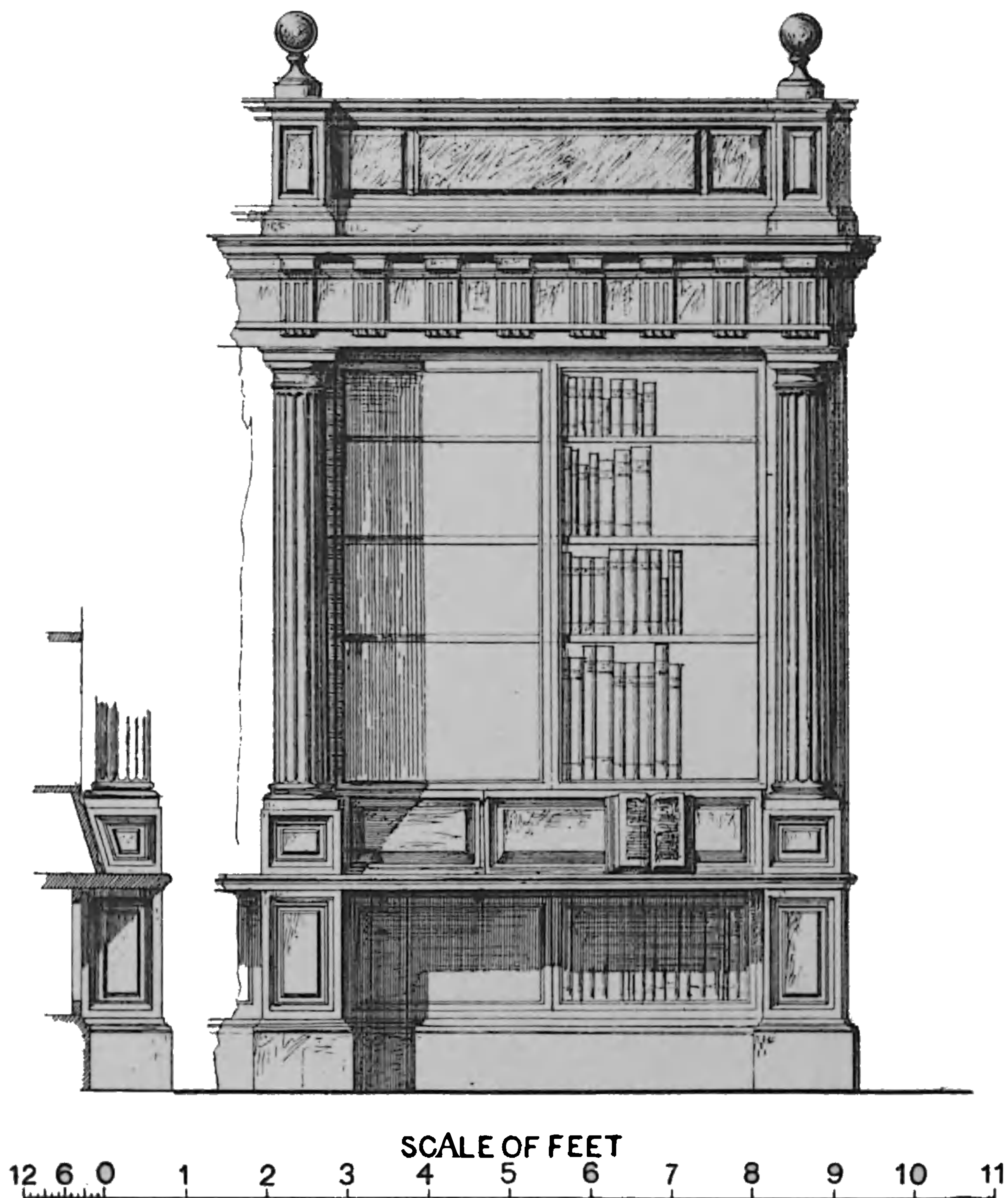
Fig. 119. Elevation of a bookcase, and section of a desk in the Library of the Escorial.
