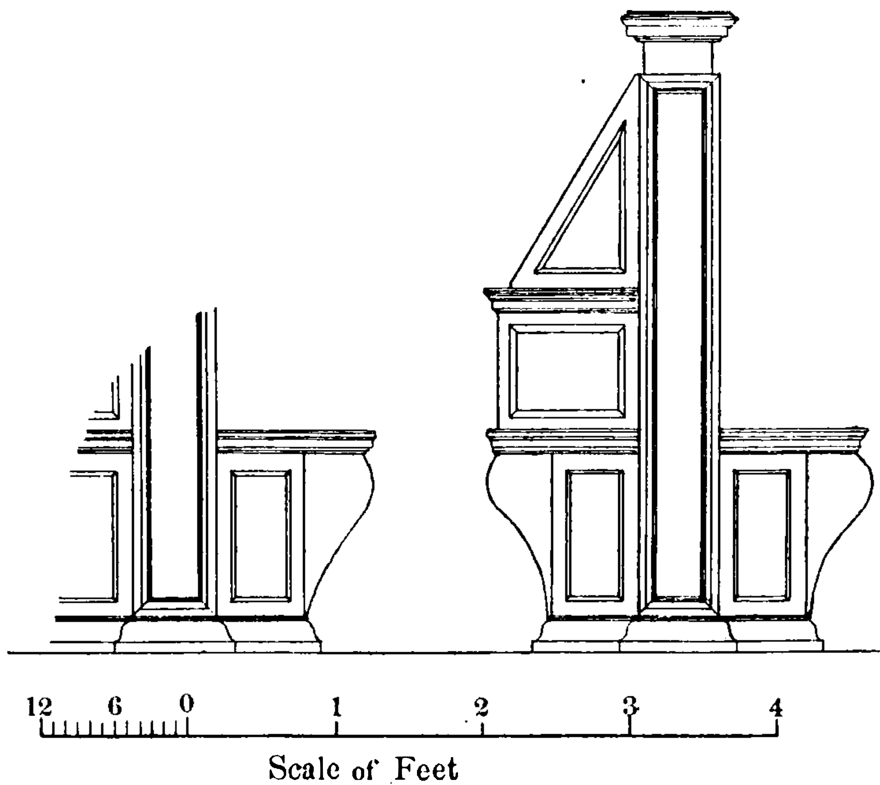
Fig. 104. Elevation of desks at Florence.
