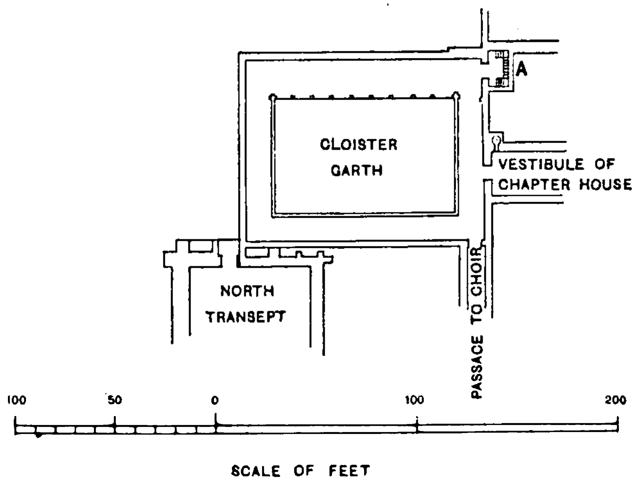
Fig. 40. Plan of the Cloister, etc., Lincoln Cathedral.
