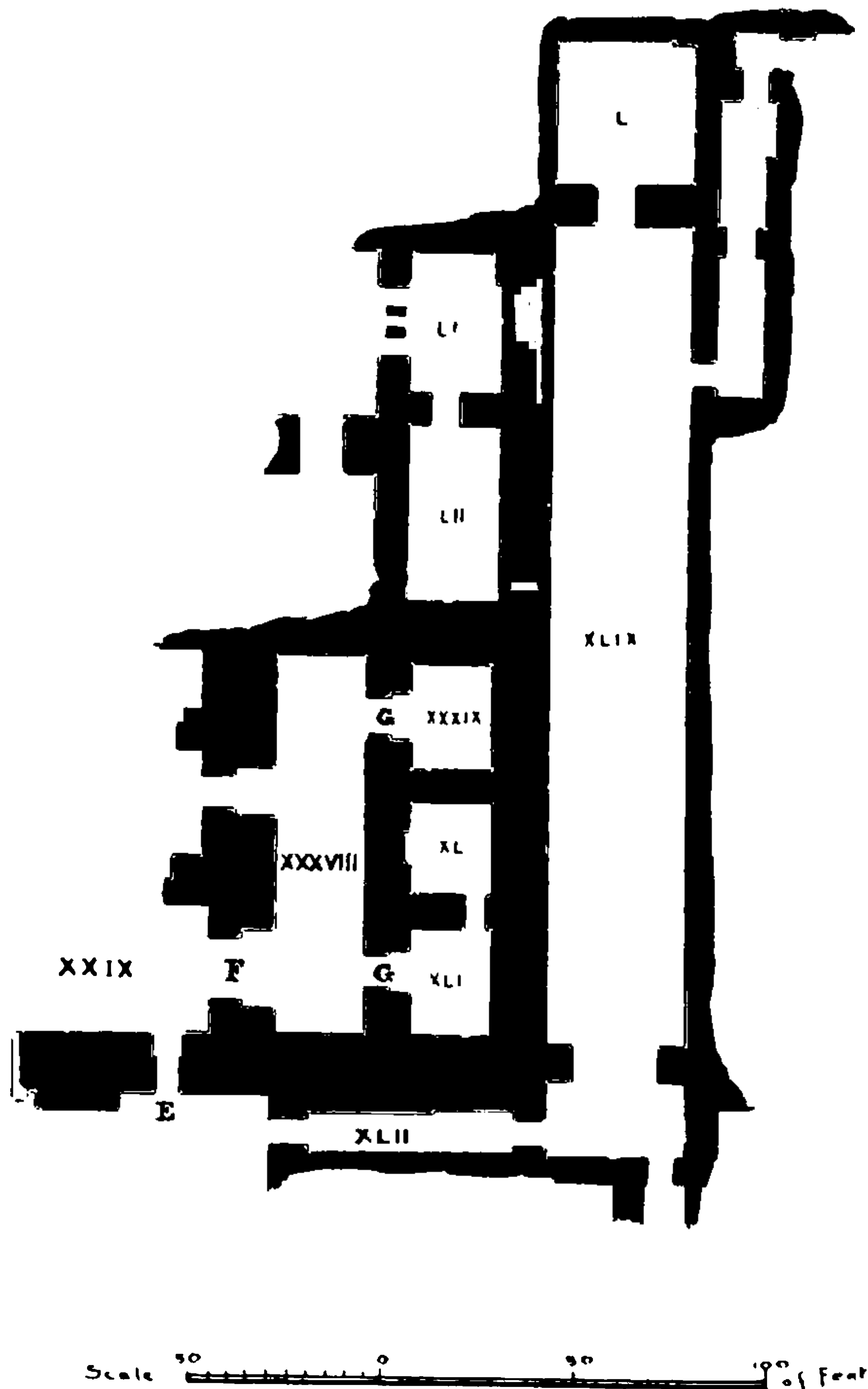
Fig. 1. Plan of the Record-Rooms in the Palace of Assur-bani-pal, King of Nineveh.
