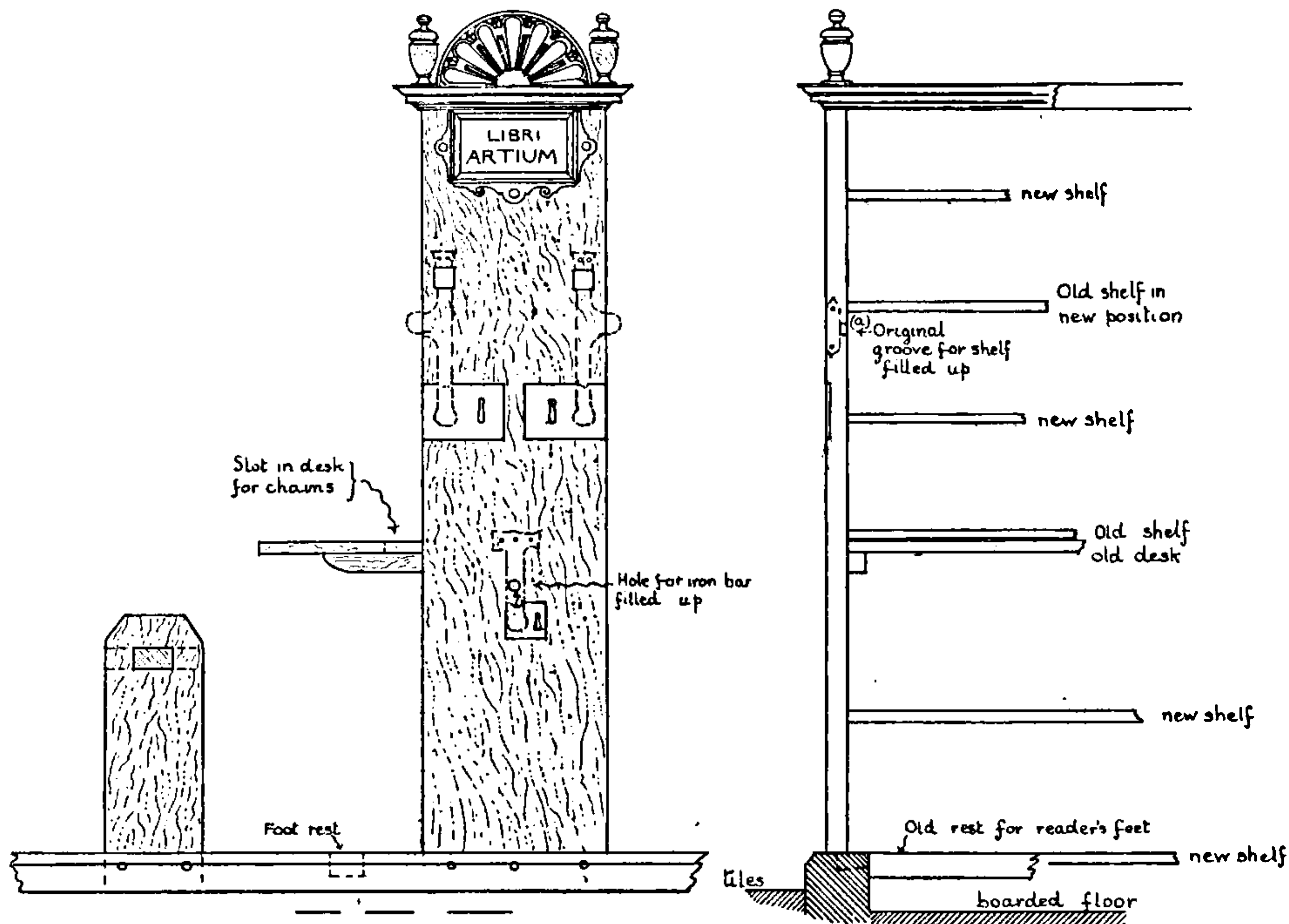
Fig. 84. Elevation of a bookcase and seat in the West Library at Merton College, Oxford.
