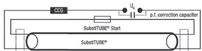
Circuit diagram of a retrofitted CCG luminaire
