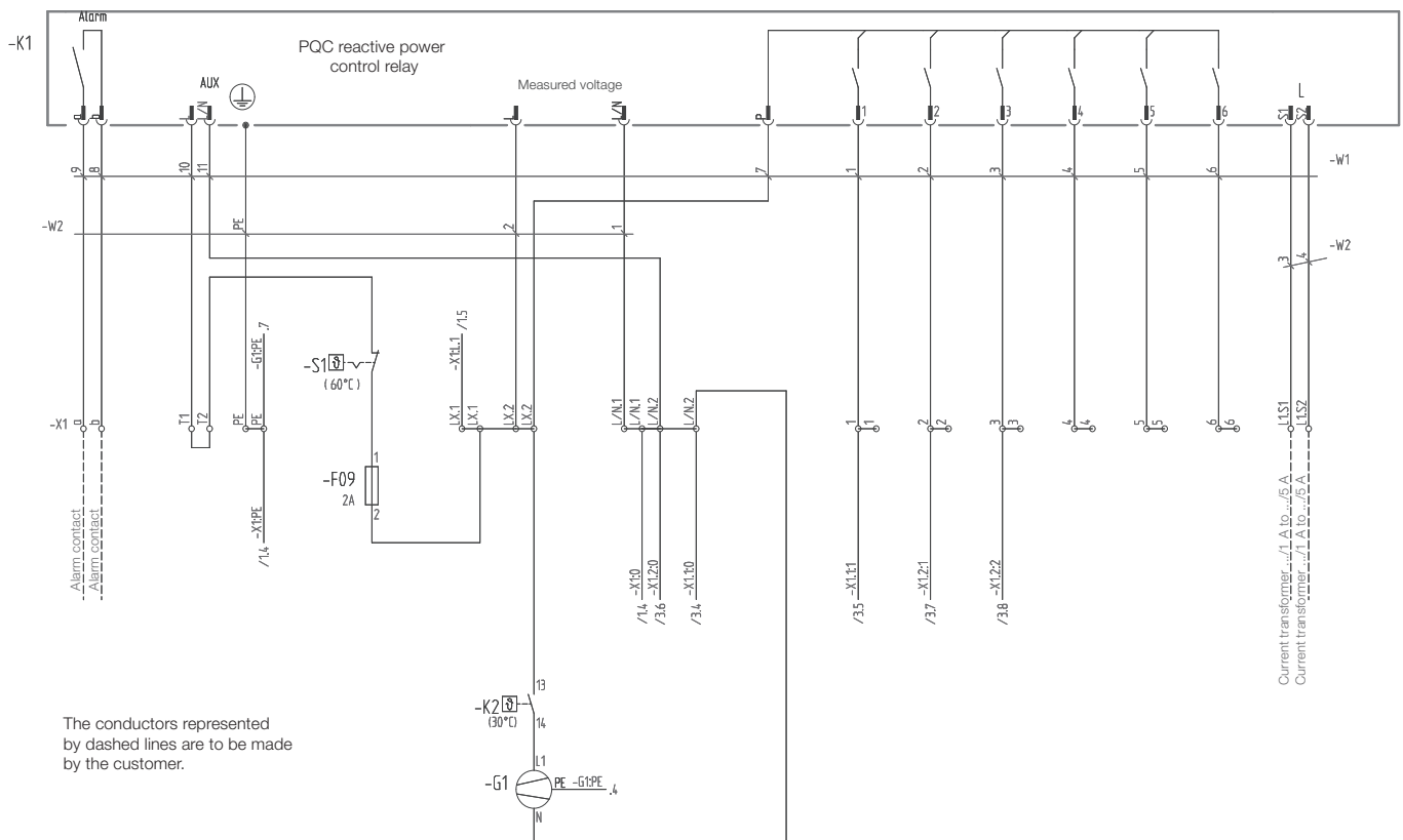
Circuit diagram of control unit (A key to the components is given on page 12.)
