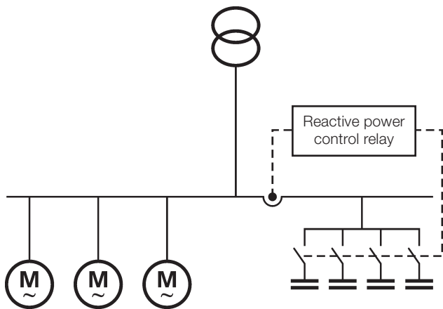
Fig. 3: Incorrect The current transformer registers zero current: the capacitor bank is not switched in. The reactive power control relay gives the message 'Undercurrent' (PQC).
