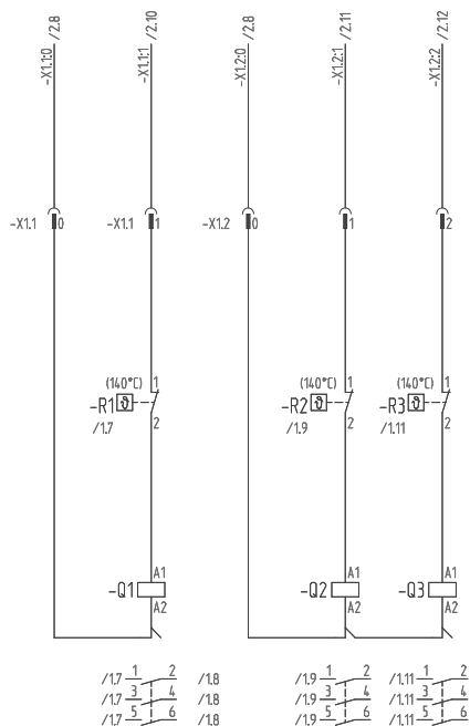
Contactor circuit diagram
