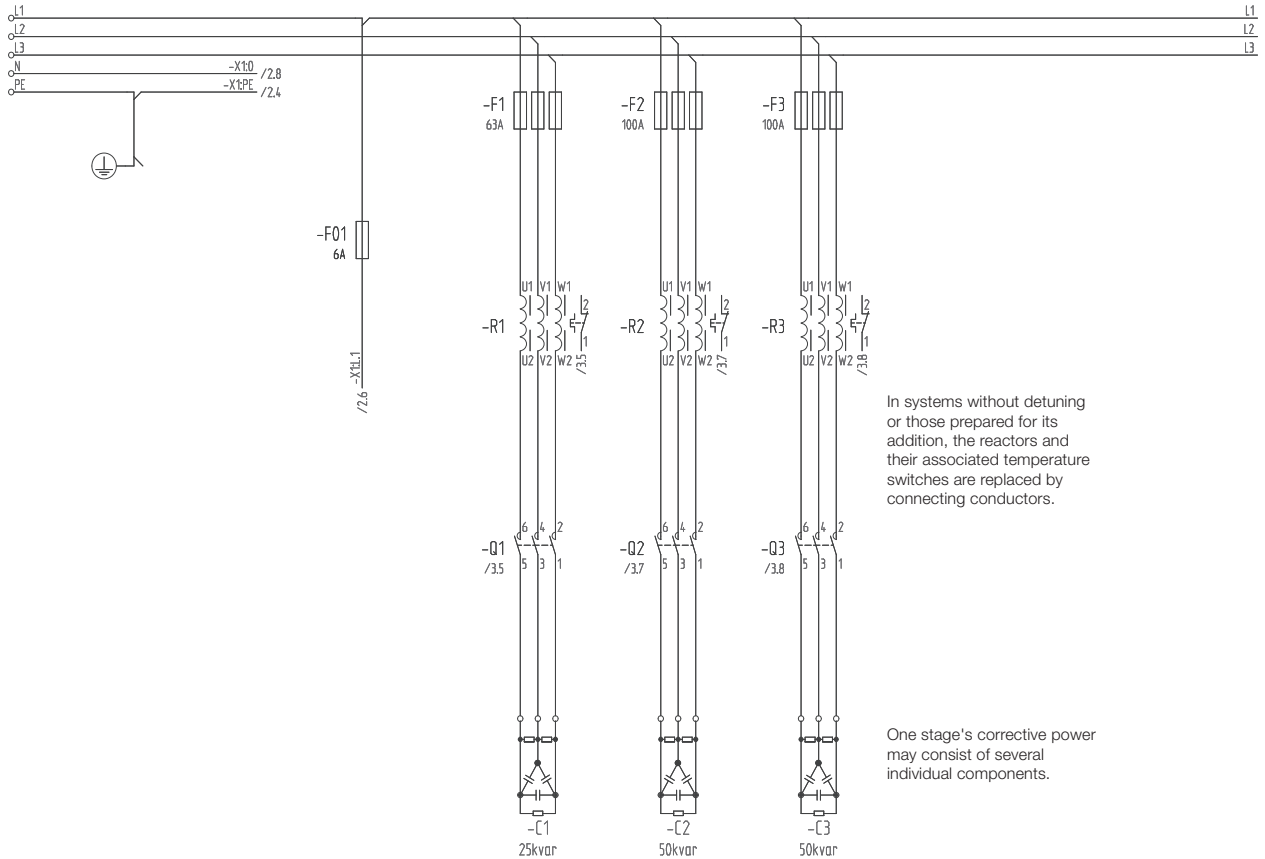
Circuit diagram of control unit (A key to the components is given on page 12.)
