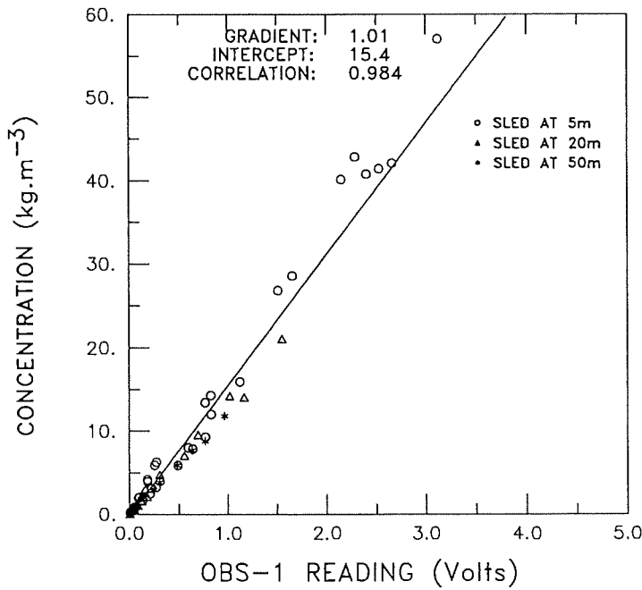
FIG.11. Sediment concentrations from water samples collected at 5, 20 and 50 m behind a Peninsula scallop dredge versus the turbidity sensor reading at Dromana.
