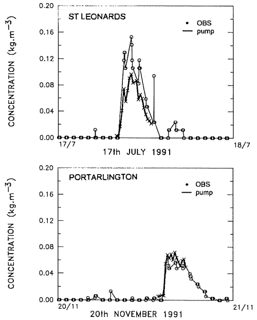
FIG.12. Comparison of sediment concentrations taken from pumped water samples and concentrations from the OBS turbidity sensors at 35 cm above the bed. The sites were downstream of experimental dredging plots at St Leonards and Portarlington.
