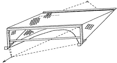
FIG.3. The New Zealand dredge.
