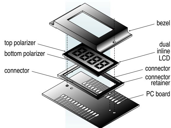
Dual Inline assembly with two ZEBRA® connectors.
