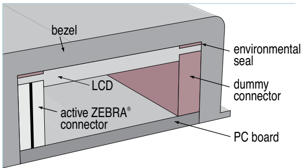
Typical Dummy ZEBBRA® installation as an environmental seal and as dummy connector.
