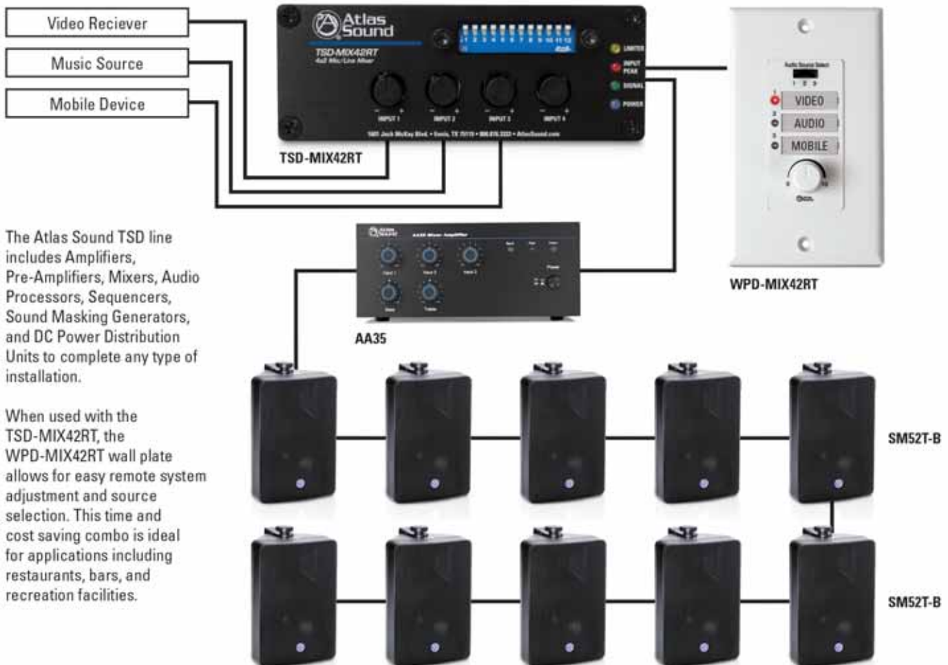
Example Restaurant/Bar Installation Using TSD-MIX42RT, WPD-MIX42RT, and AA35 Amplifier
