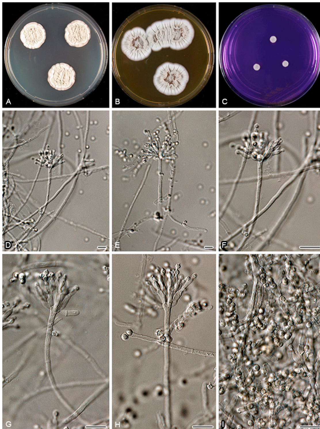
Fig. 5. Aspergillus inflatus . A. Colonies on CYA. B. Colonies on MEA. C. Colonies on CREA. D–H. Conidiophores. I. Conidia. Scale bars: D–I = 10 \mu m.
