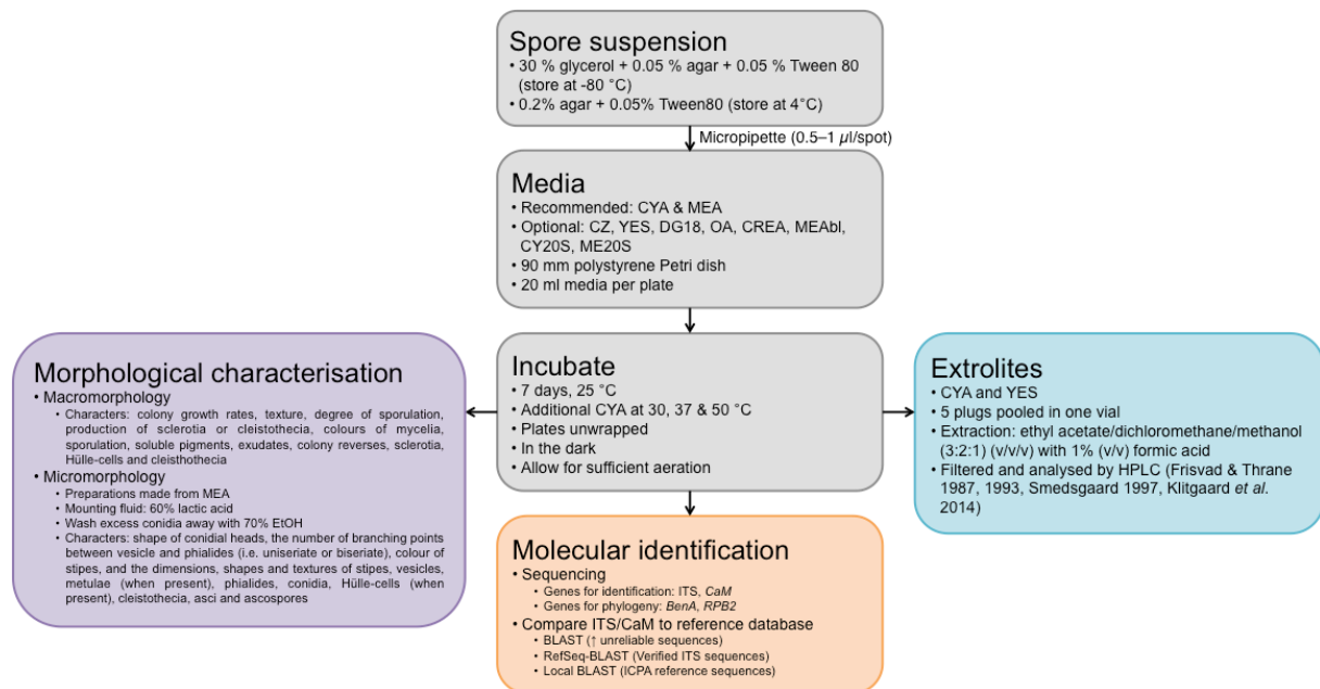
Fig. 2. Flow diagram summarising recommended methods for the identification and characterization of Aspergillus .
