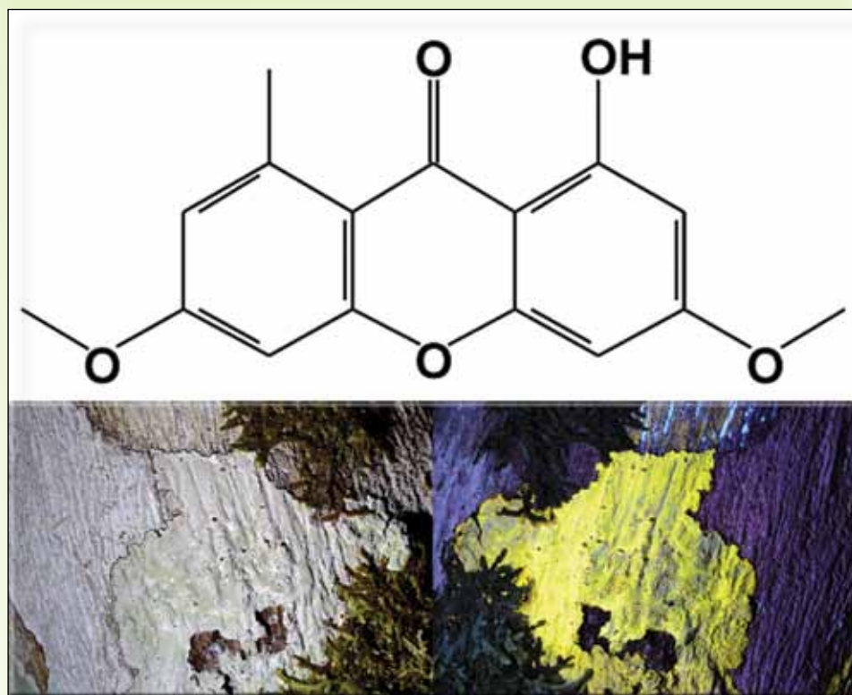
Figure 4. Lichexanthone is the most common lichen “sunscreen.” It “glows” bright yellow under long-wave UV light (here shown with the lichen Diorygma epiglaucum ). This is caused by the two “aromatic” rings of the molecule, formed by unsaturated double bonds. These bonds absorb long-wave UV radiation and transform it into visible light at lower energy, thus avoiding damage to the lichen harmful UV radiation. Graphic and photos R. Lücking.
