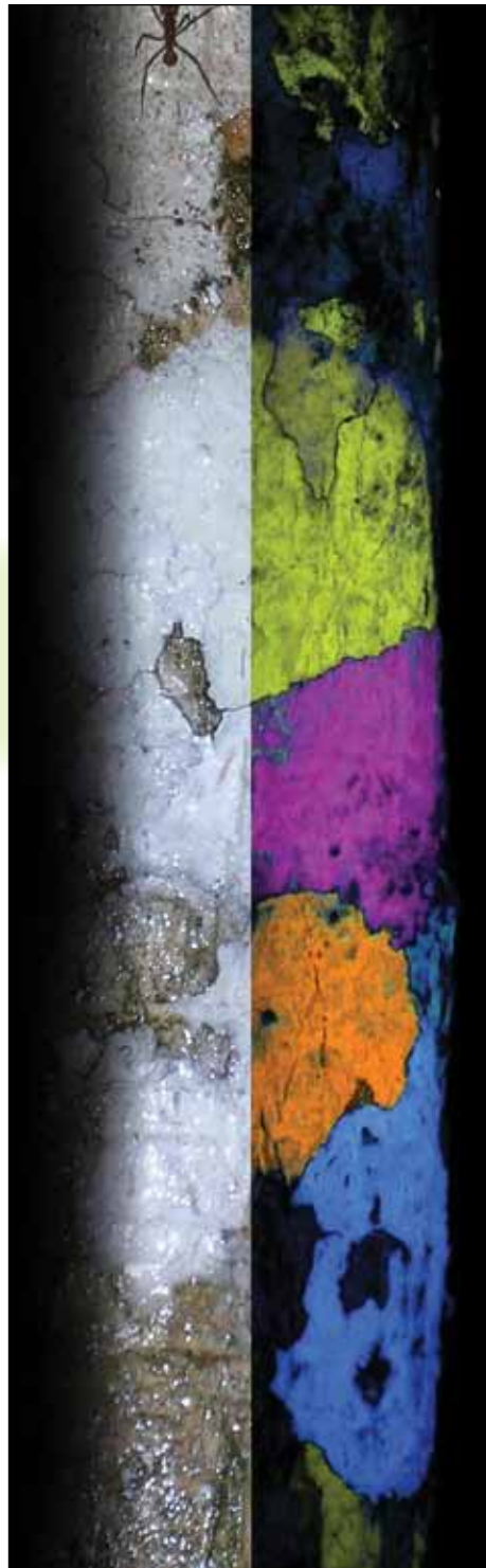
Figure 2. Stem of a small tropical tree at Las Cruces Biological Station in Costa Rica, photographed at night under normal light (left half) and under 354 nm long-wave UV light (right half). Photos R. Lücking.
