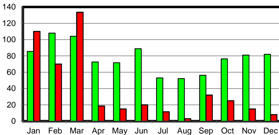
Figure 2. 2019 Monthly rainfall at Wandella (red); 130 year average (green).
