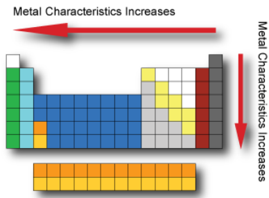
Figure 8. Position of HMs in periodic table https://www.modelscience.com/PeriodicTable.html
