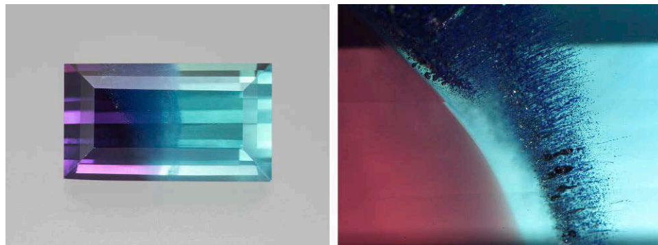
Figure 51. Left: Bicolor 14.83 ct synthetic sapphire showing popular teal blue and purple colors. Photo by Kevin Schumacher; courtesy of RusGems. Right: Wisps of presumably \text{CoAl}_2\text{O}_4 at the boundary of the teal and purple colors in the crystal. Photomicrograph by Nathan Renfro; field of view 7.05 mm.
