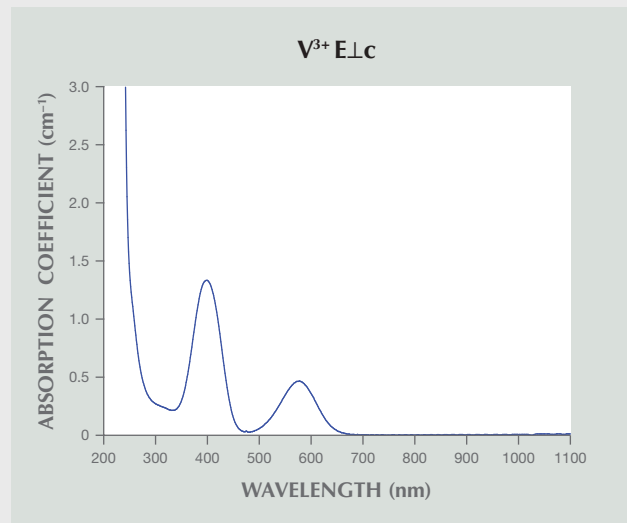
Figure A-3. UV-Vis-NIR infrared absorption coefficient spectrum of the V^{3+} -doped synthetic sapphire, produced by dividing the spectrum in figure A-2 by sample thickness (0.626 cm) and multiplying by 2.303. Note that the shape of the curve is the same but the y-axis units are cm^{-1} .
