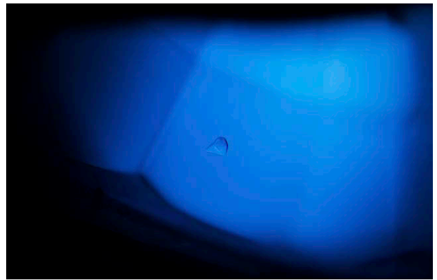
Figure 1. This small transparent colorless crystal in spinel was identified by Raman analysis as actinolite. Photomicrograph by E. Billie Hughes; field of view 1.7 mm.
