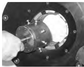
Insert die set in crimper.
