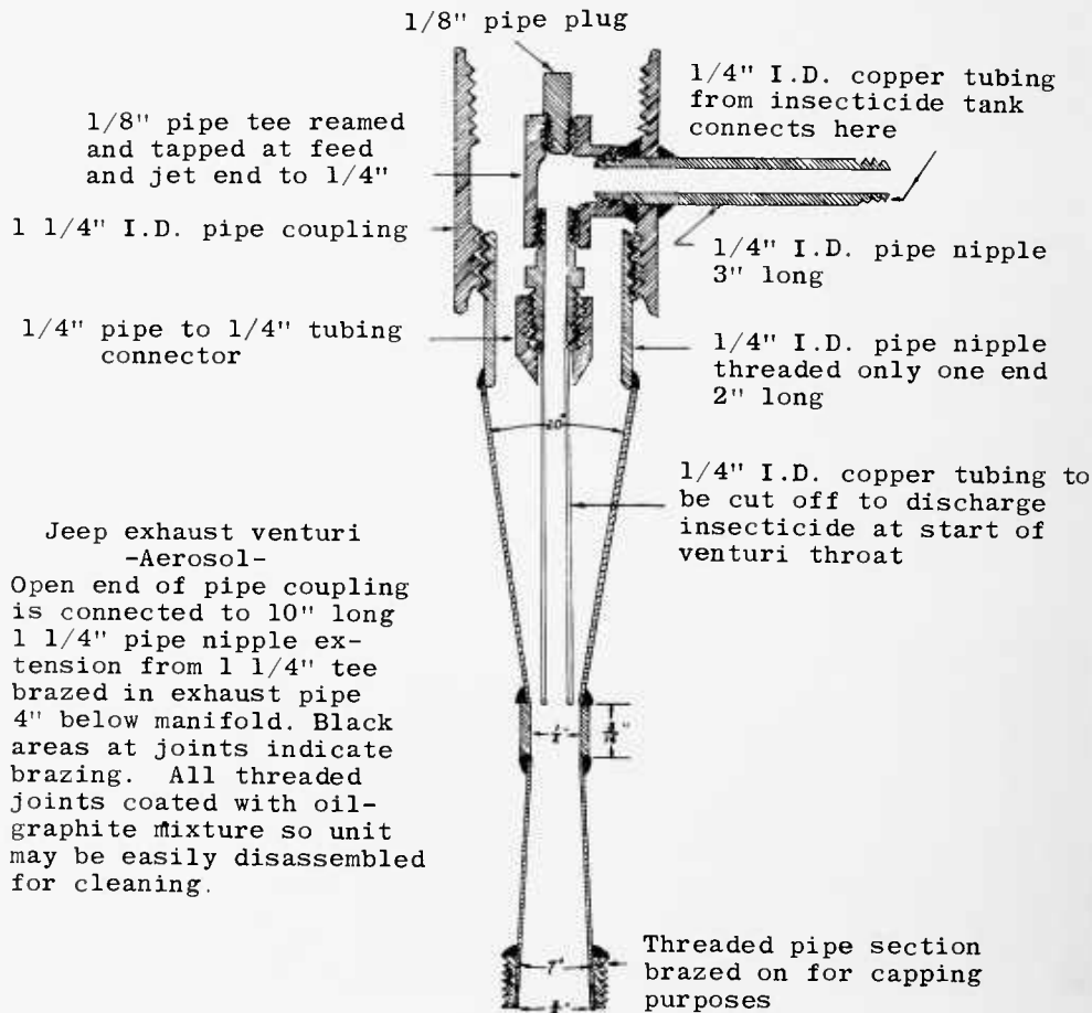
FIGURE 23.—Diagram of a jeep exhaust venturi aerosol. (From Jones and Holten 78.)
