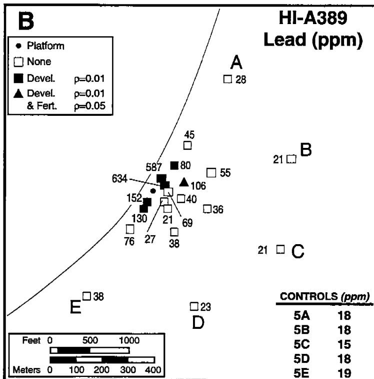
Figure 6.62. Whole sediment A: zinc; and B: lead concentrations and pore water toxicity at HI-A389. (Devel.=standard sea urchin developmental assay; Fert.=standard sea urchin embryo fertilization assay).
