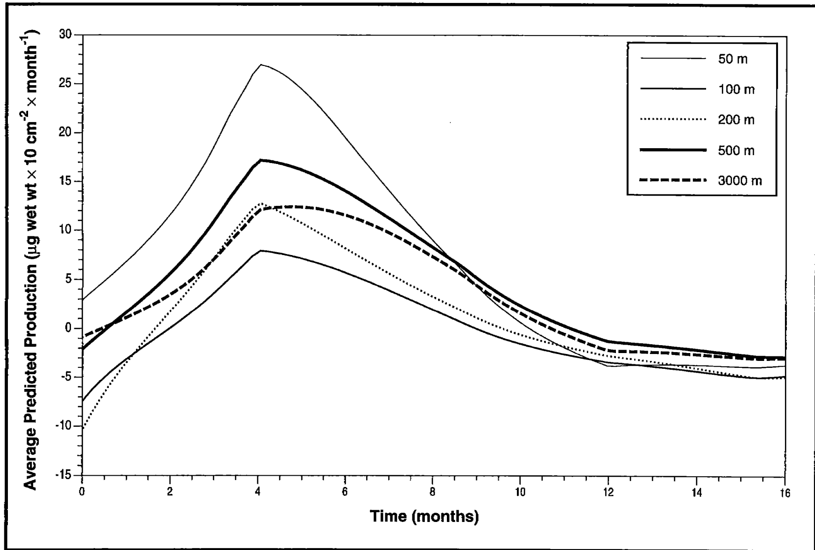
Figure 5.99. Average predicted production for the meiofaunal community at MU-A85 over the timeframe of the study sampling efforts (0=February 1993).
