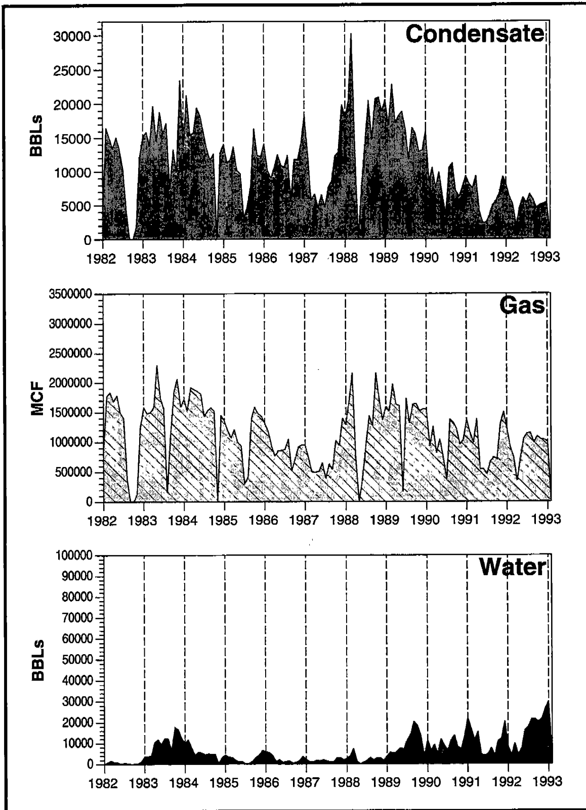
Figure 1.6. Monthly production of condensate, gas, and water at MU-A85.
