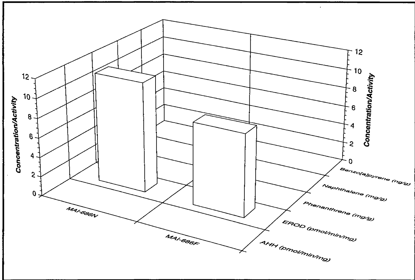
Figure 5.126. Catalytic enzyme activities and biliary metabolite concentrations in Ancyloperetta quadrocellata .
