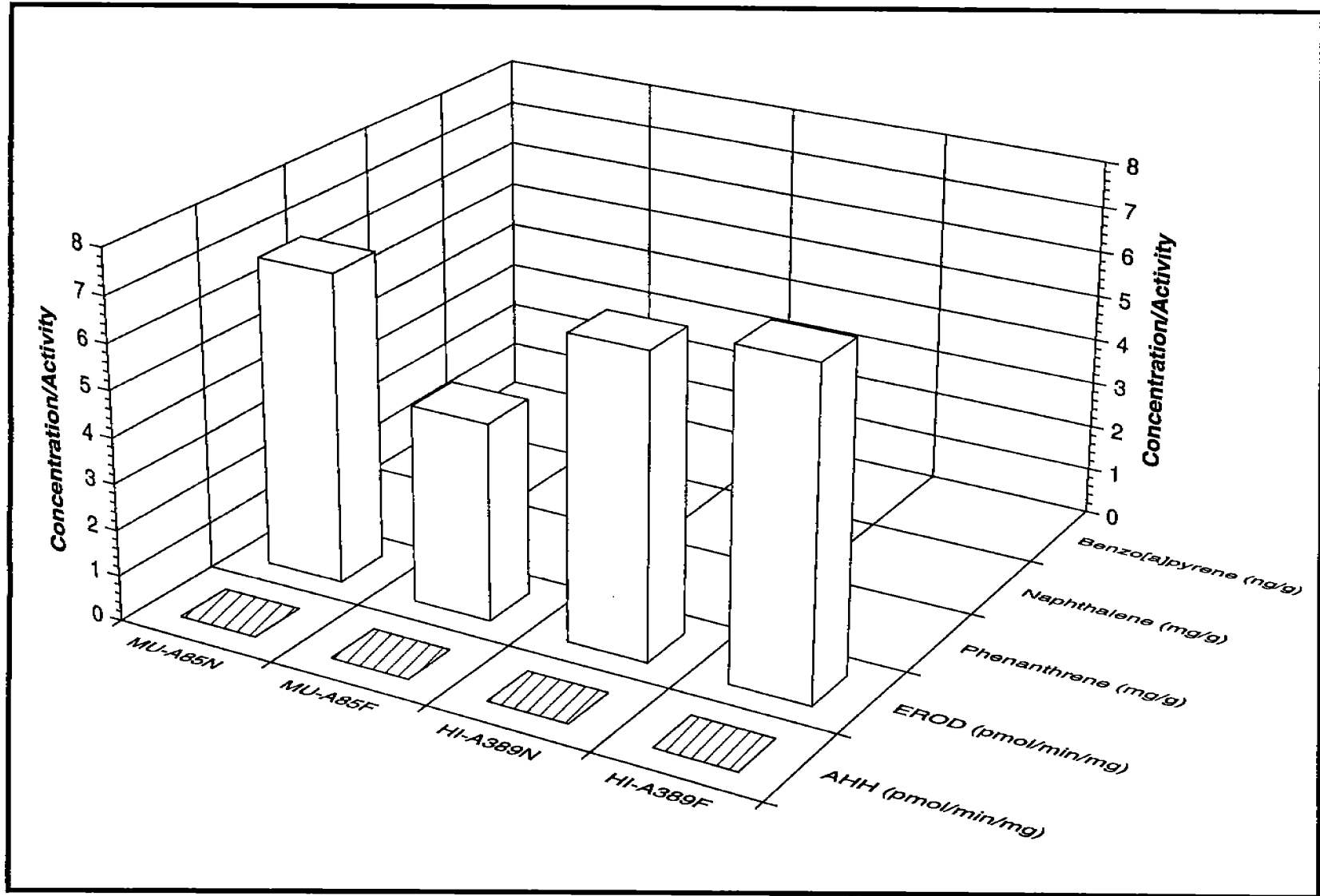
Figure 5.125. Catalytic enzyme activities and biliary metabolite concentrations in Ancylopussetta dilecta .
