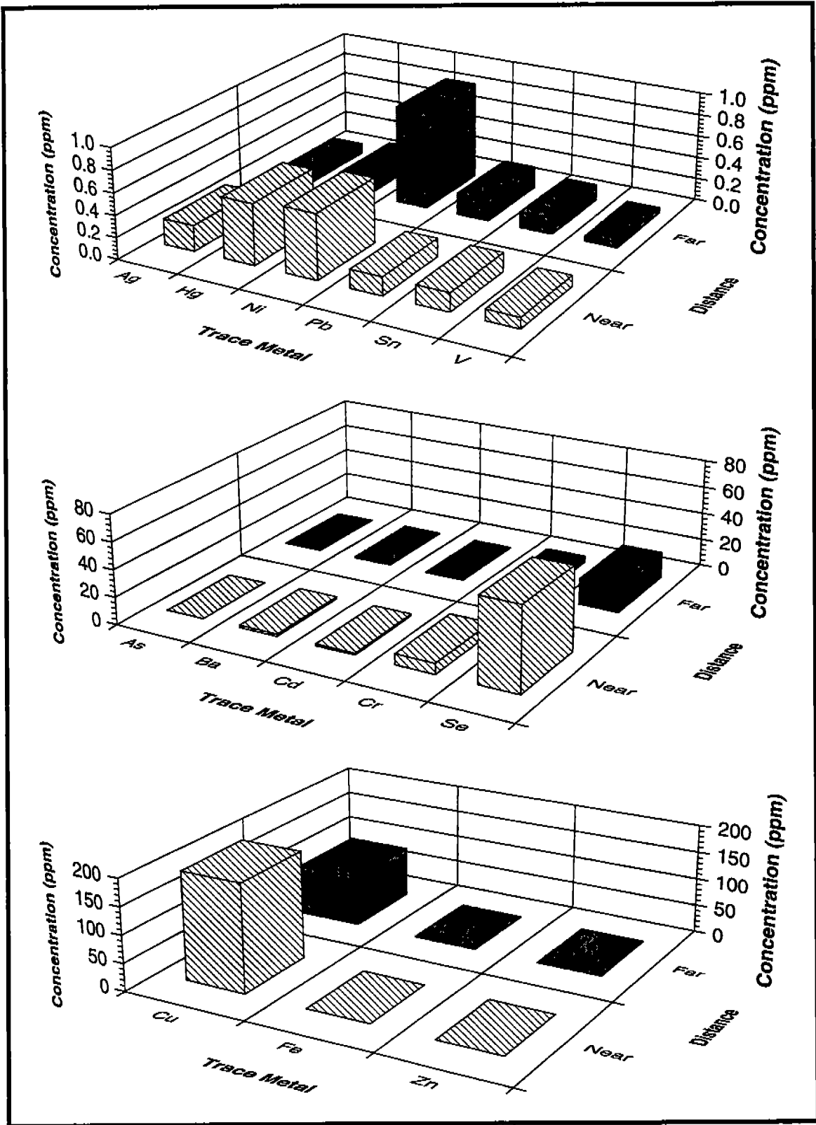
Figure 5.75. Summary of mean metal concentrations in fish liver tissues at MAI-686 as a composite of all four cruises.
