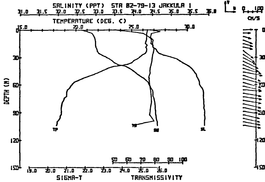
Figure XIV-5. Plot of salinity (SL), temperature (TP), transmissivity (TR), and sigma-t (SG) from Jakkula 1.
