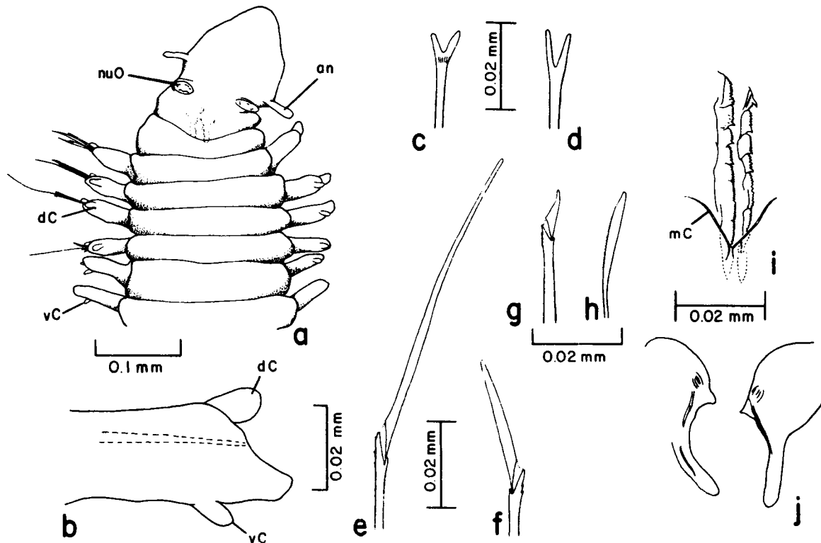
Figure 44-30. Meiodorvillea sp. B: a, anterior end; b, parapodium from setiger 2 (posterior view); c, furcate seta from setiger 3; d, same, from posterior setiger; e, upper compound seta; f, middle compound seta; g, lower compound seta; h, inferior simple seta; i, entire maxillae (dorsal view); j, mandibles (dorsal view).
