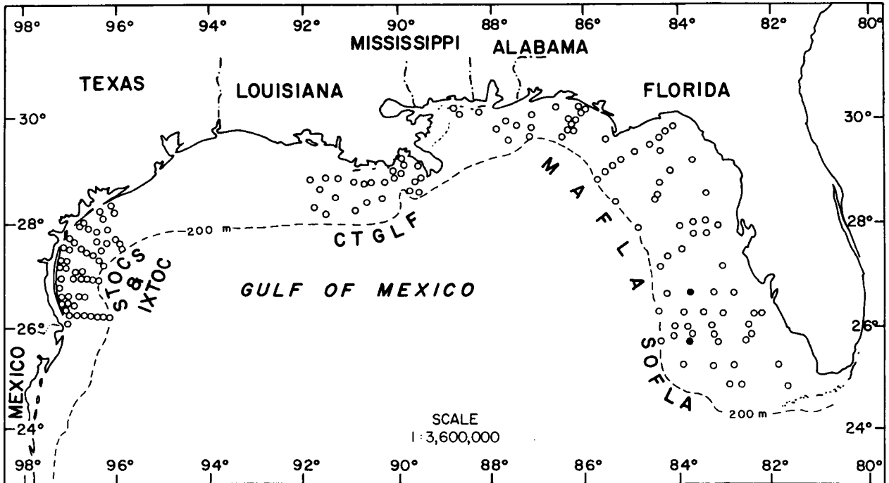
Figure 39-13. Distribution of Ramphobrachium diversosetosum on the outer continental shelf of the northern Gulf of Mexico based on its occurrence (●) in BLM-OCS monitoring programs.
