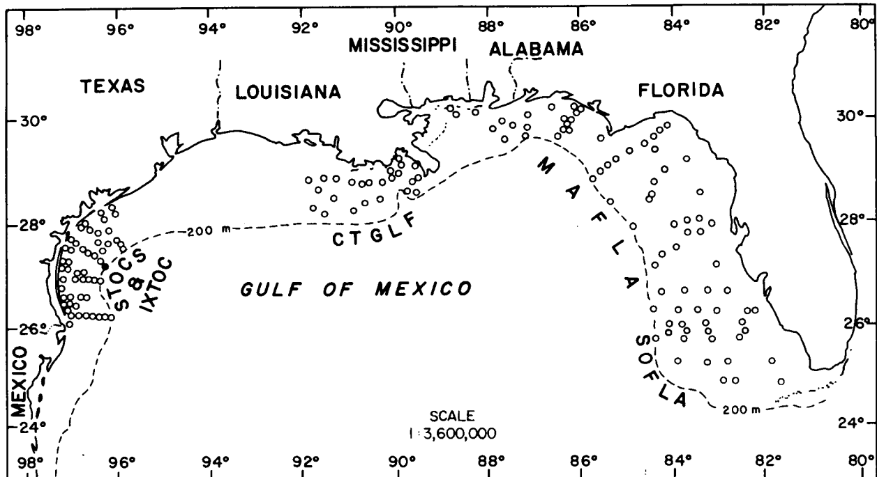
Figure 41-15. Distribution of Lumbrineris brevipennis on the outer continental shelf of the northern Gulf of Mexico based on its occurrence (●) in BLM-OCS monitoring programs.
