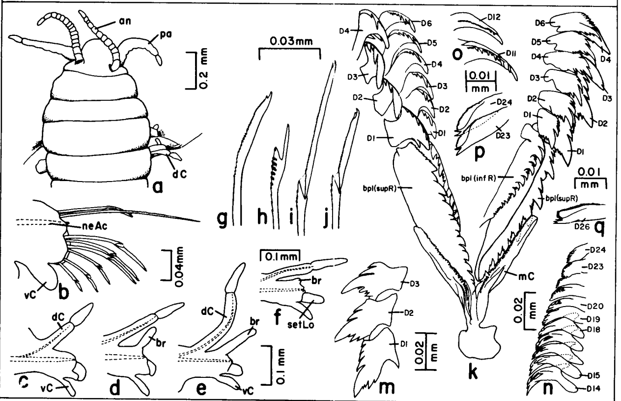
Figure 44-16. Schistomeringos cf. rudolphi : a, anterior end; b, parapodium from setiger 1 (posterior view); c, parapodium from setiger 4 (posterior view); d, parapodium from setiger 6 (posterior view); e, parapodium from setiger 9 (posterior view); f, parapodium from setiger 16 (posterior view); g, cultriform seta; h, furcate seta; i, upper compound falciger; j, lower compound falciger; k, posterior portion of maxillae (dorsal view); m, free denticles 1-3 from superior row; n, free denticles 14-24 from superior row; o, free denticles 11, 12 from inferior row; p, free denticles 23, 24 from inferior row; q, free denticle 26 from inferior row.
