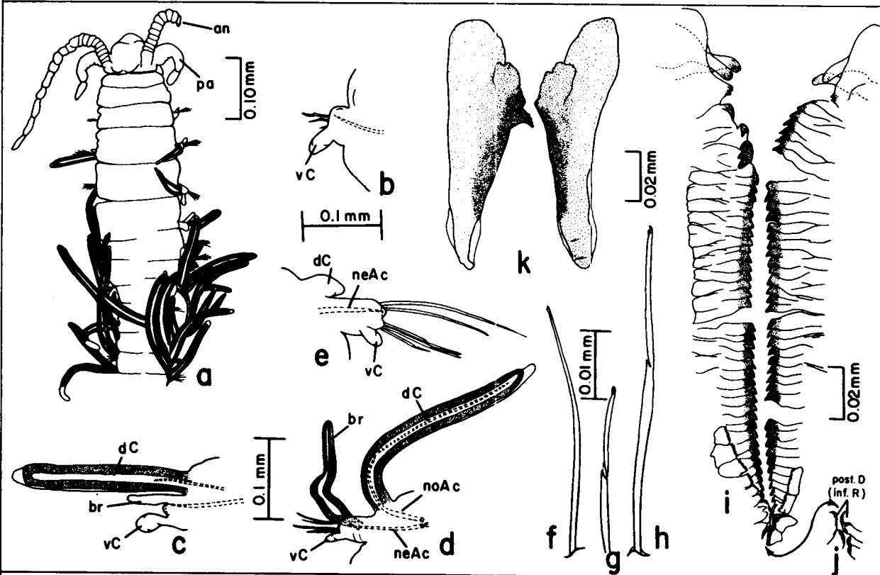
Figure 44-24. Genus B: a, anterior end; b, parapodium from setiger 1 (anterior view); c, parapodium from setiger 4 (anterior view); d, parapodium from mid-branchiate region (anterior view); e, posterior parapodium (posterior view); f, simple supra-acicular seta; g, subacicular compound falciger; h, subacicular pseudocompound falciger from far posterior region; i, entire maxillae (dorsal view); j, posteriormost denticles (inferior row); k, mandibles (dorsal view).
