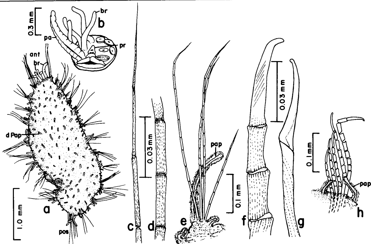
Figure 47-4. Diplocirrus sp. A: a, whole worm (dorsal view); b, introvert (branchiae and palp from right side removed); c, distal end of notoseta; d, median section of notoseta; e, notopodium from setiger 10; f, distal end of neuroseta; g, pseudocompound falciger from last neuropodium; h, neuropodium from setiger 10.
