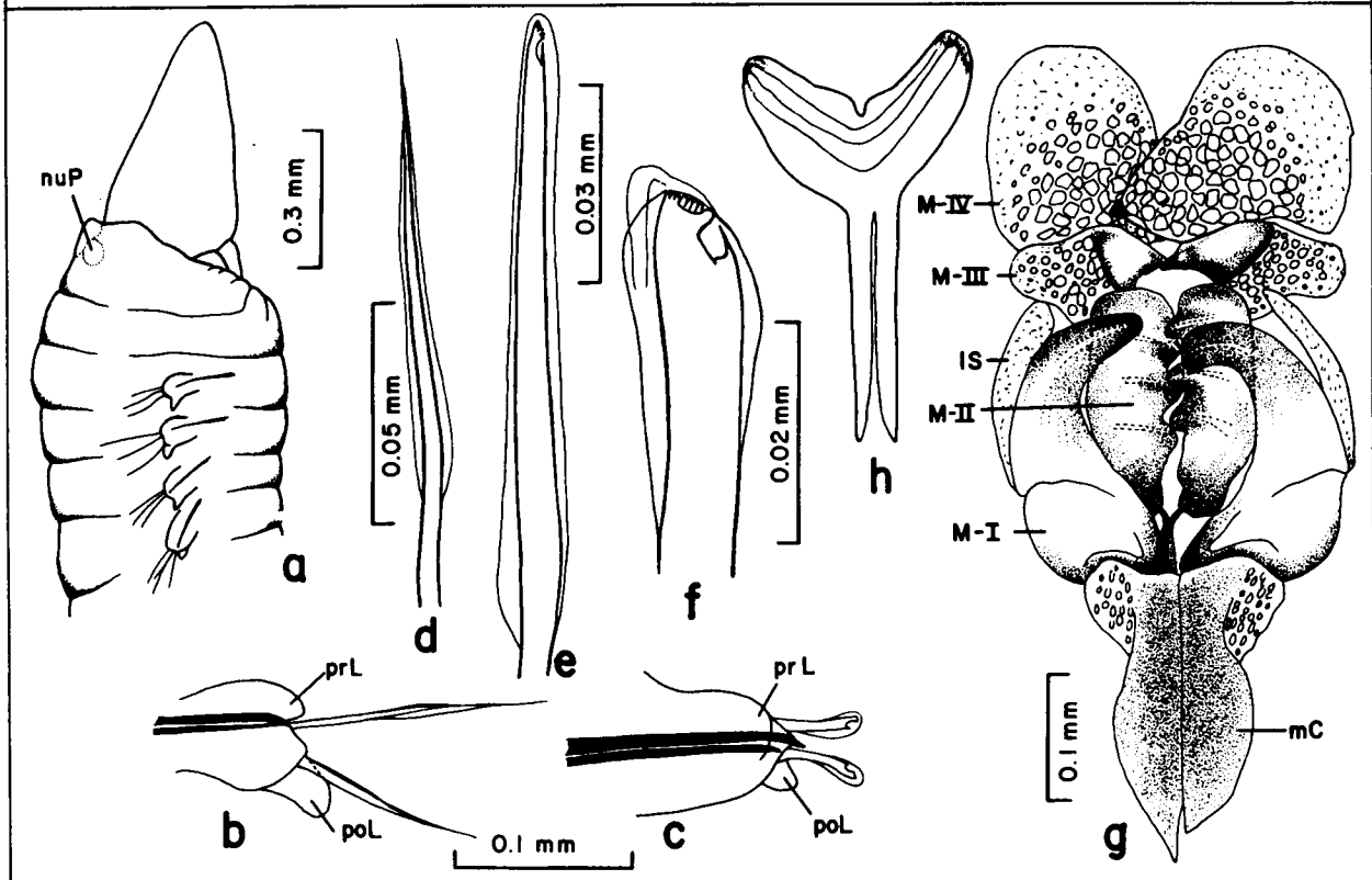
Figure 41-16. Lumbrineris brevipennis : a, anterior end (lateral view); b, parapodium from setiger 2; c, parapodium from setiger 22 (anterior view); d, limbate seta from setiger 2; e, hooded hook from setiger 4; f, same, from setiger 23; g, maxillae; h, mandibles (from USNM 33765; no scale).
