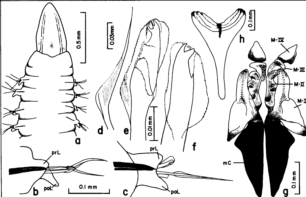
Figure 41-6. Lumbrinerides sp. A: a, anterior end; b, parapodium from setiger 5; c, parapodium from setiger 10; d, limbate seta from setiger 10; e, composite hooded hook from setiger 3; f, simple hooded hook from setiger 7; g, maxillae; h, mandibles.
