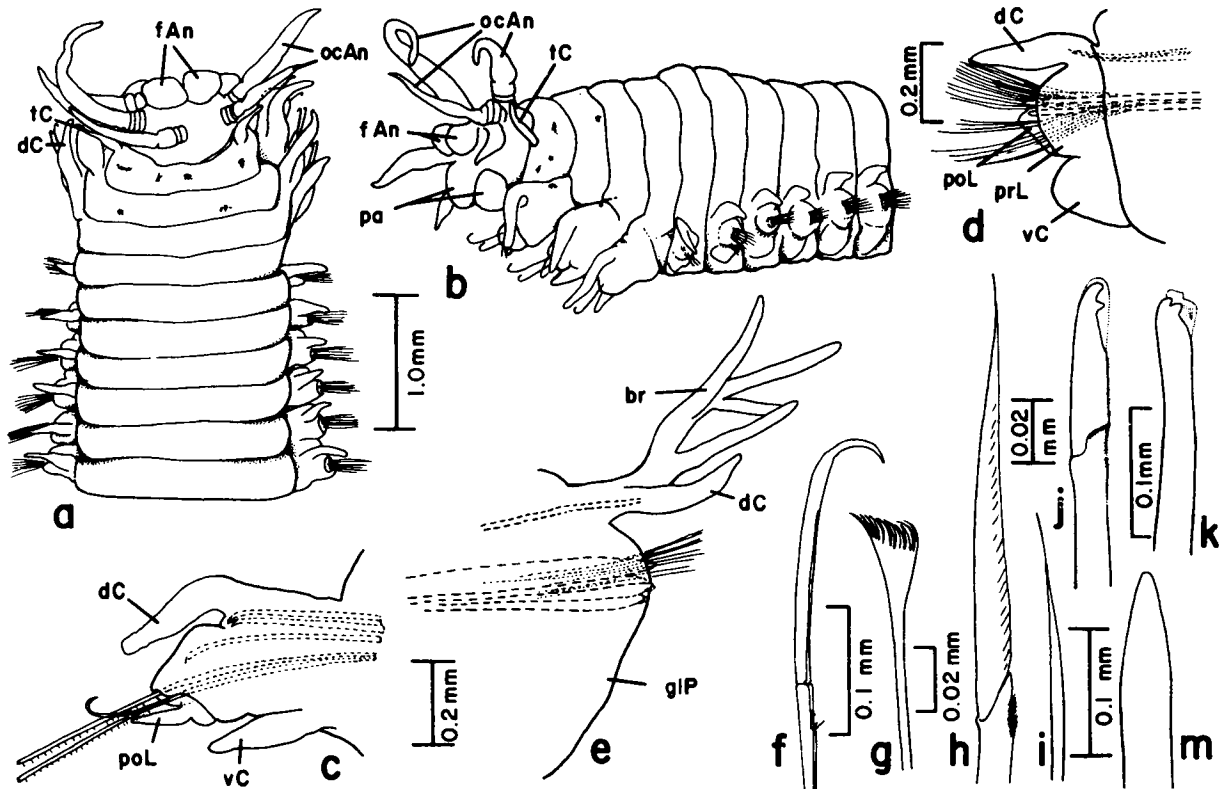
Figure 39-14. Ramphobrachium diversosetosum : a, anterior end, dorsal view; b, same, lateral view; c, parapodium from setiger 2; d, same, from setiger 5; e, same, from setiger 25; f, modified hook from setiger 2; g, pectinate seta; h, compound spiniger from setiger 4; i, limbate seta; j, compound falciger from setiger 4; k, sub-acicular hook; m, aciculum.
