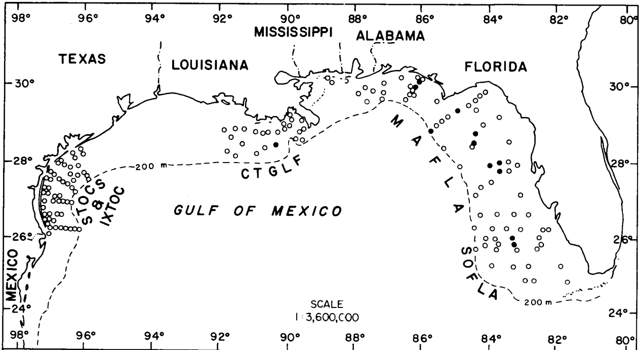
Figure 44-15. Distribution of Schistomeringos cf. rudolphi on the outer continental shelf of the northern Gulf of Mexico based on its occurrence (●) in BLM-OCS monitoring programs.
