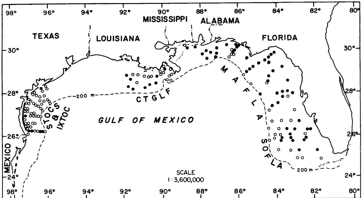
Figure 39-19. Distribution of Mooreonuphis cf. nebulosa on the outer continental shelf of the northern Gulf of Mexico based on its occurrence (●) in BLM-OCS monitoring programs.
