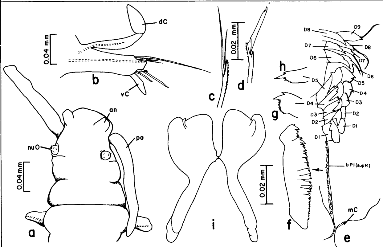
Figure 44-12. Schistomerings sp. B: a, anterior end (antennae presumed broken); b, anterior parapodium (posterior view); c, furcate seta; d, middle compound falciger; e, entire left side of maxillae (dorsal view); f, left basal plate (lateral view); g, free denticle 4 from superior row; h, free denticle 5 from superior row; i, mandibles (dorsal view).
