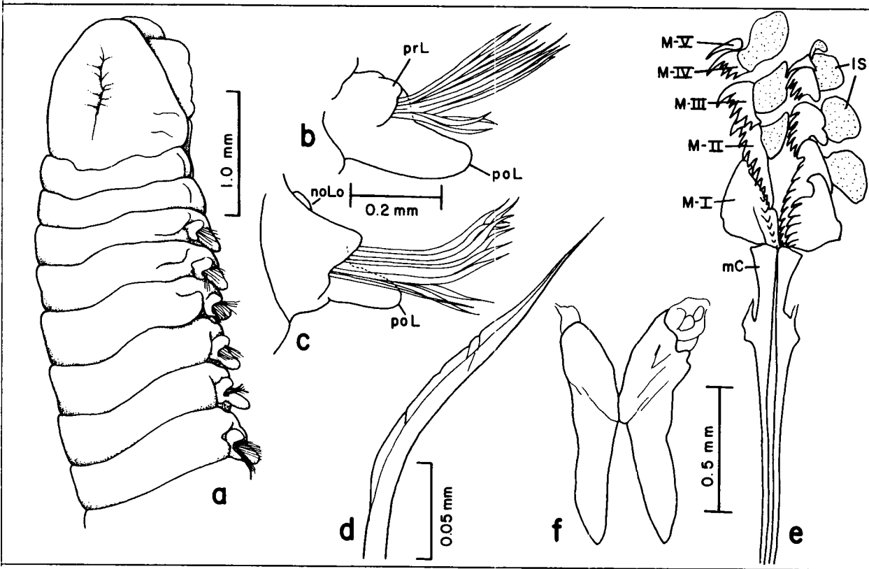
Figure 42-2. Arabella iricolor : a, anterior end; b, parapodium from setiger 8 (anterior view); c, parapodium from midbody region (anterior view); d, limbate seta from midbody region; e, maxillae; f, mandibles (ventral view).
