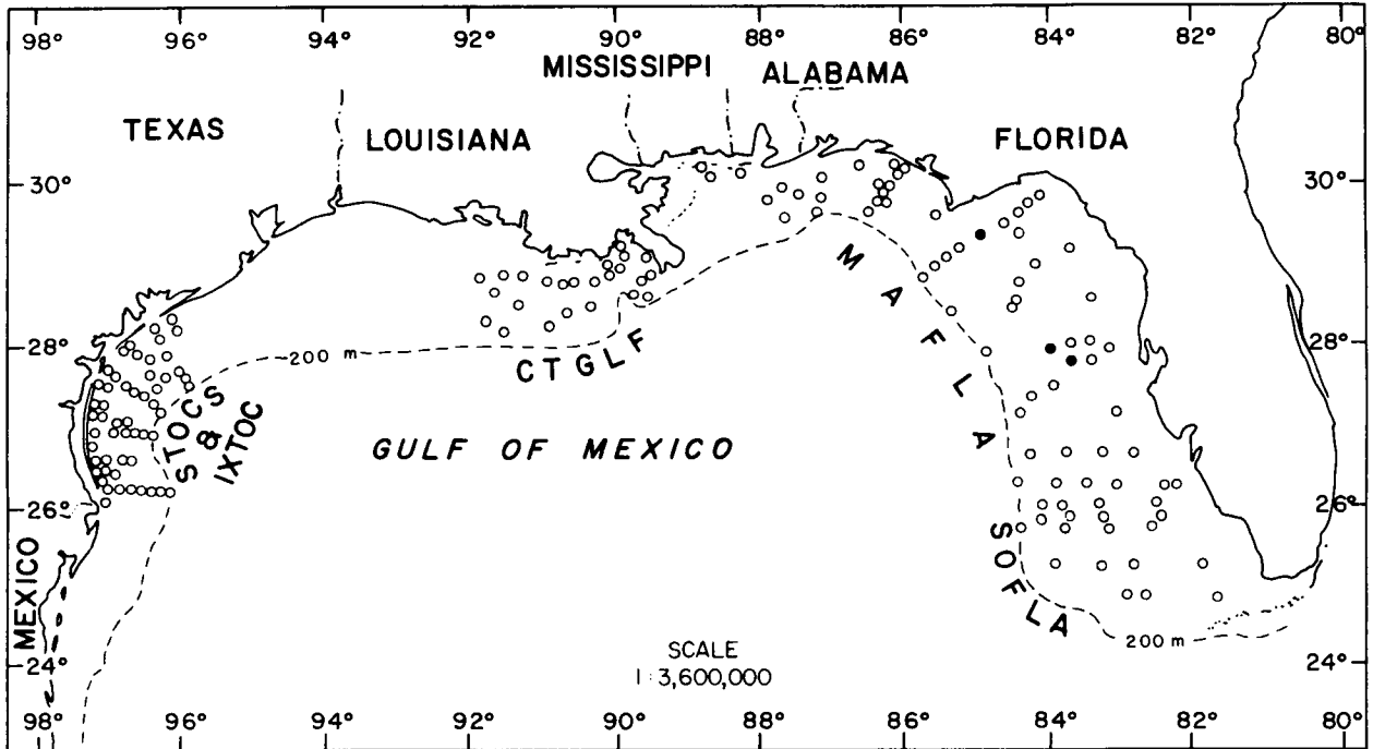
Figure 44-11. Distribution of Schistomerings sp. B on the outer continental shelf of the northern Gulf of Mexico based on its occurrence (●) in BLM-OCS monitoring programs.
